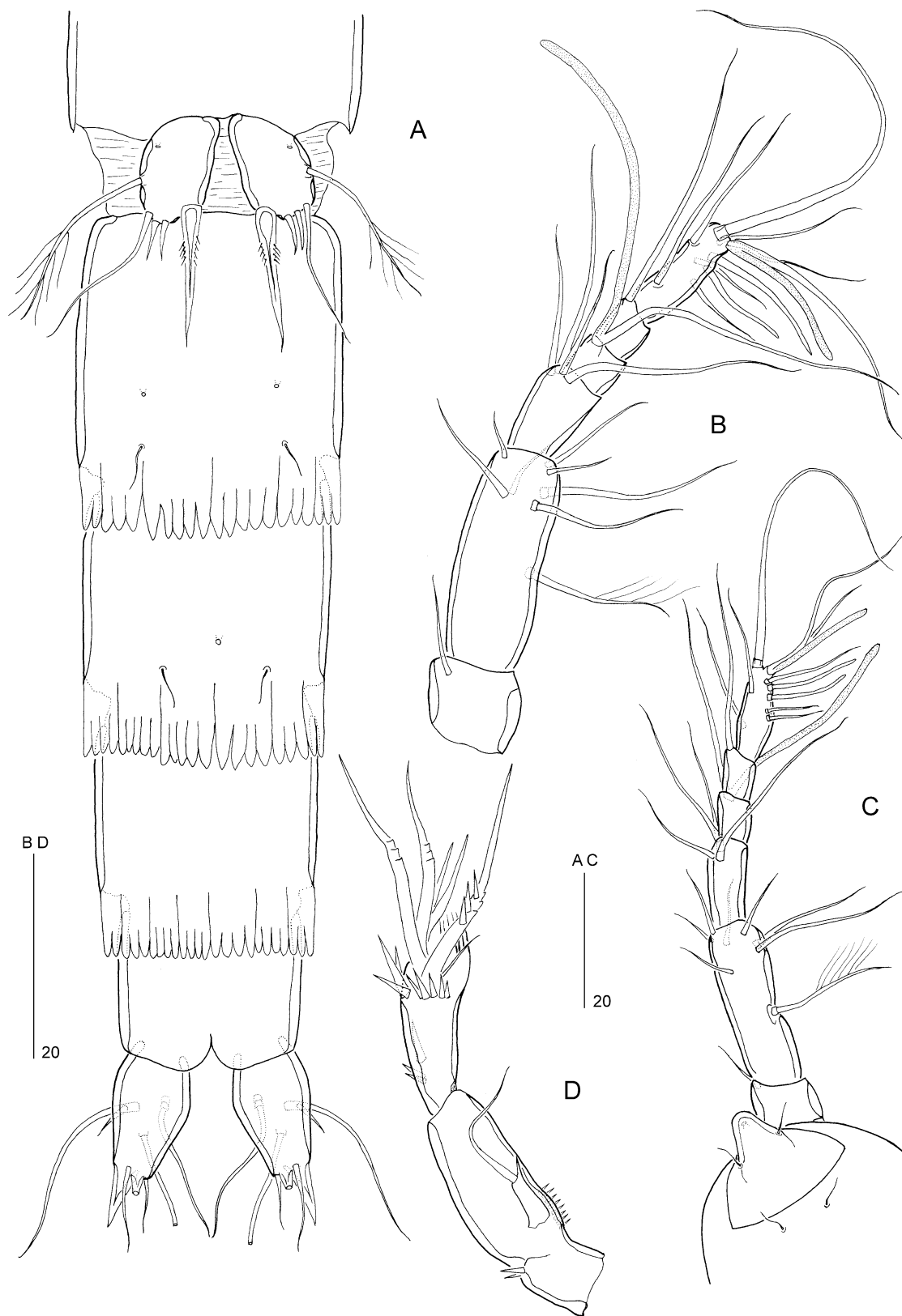
Figure 19. Mesopontia dillonbeachia (Lang, 1965) comb. nov. (♀). A, urosome, ventral view. B, antennule, ventral view. C, rostrum and antennule, dorsal view. D, antenna.
