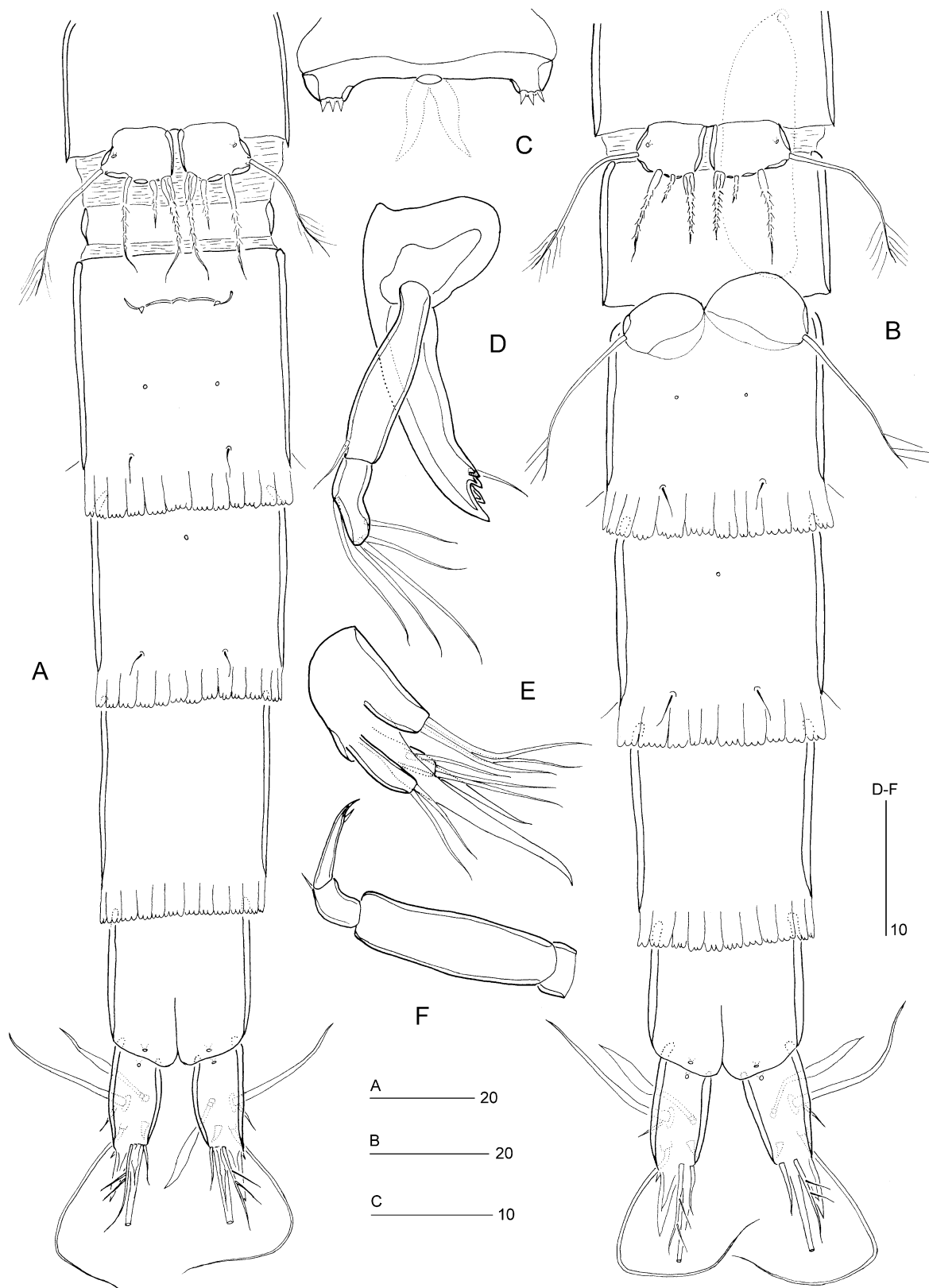
Figure 2. Arenopontia nesaie Cottarelli, 1975. A, urosome ♀, ventral view. B, urosome ♂, ventral view. C, genital field ♀. D, mandible. E, maxilla. F, maxilliped.
