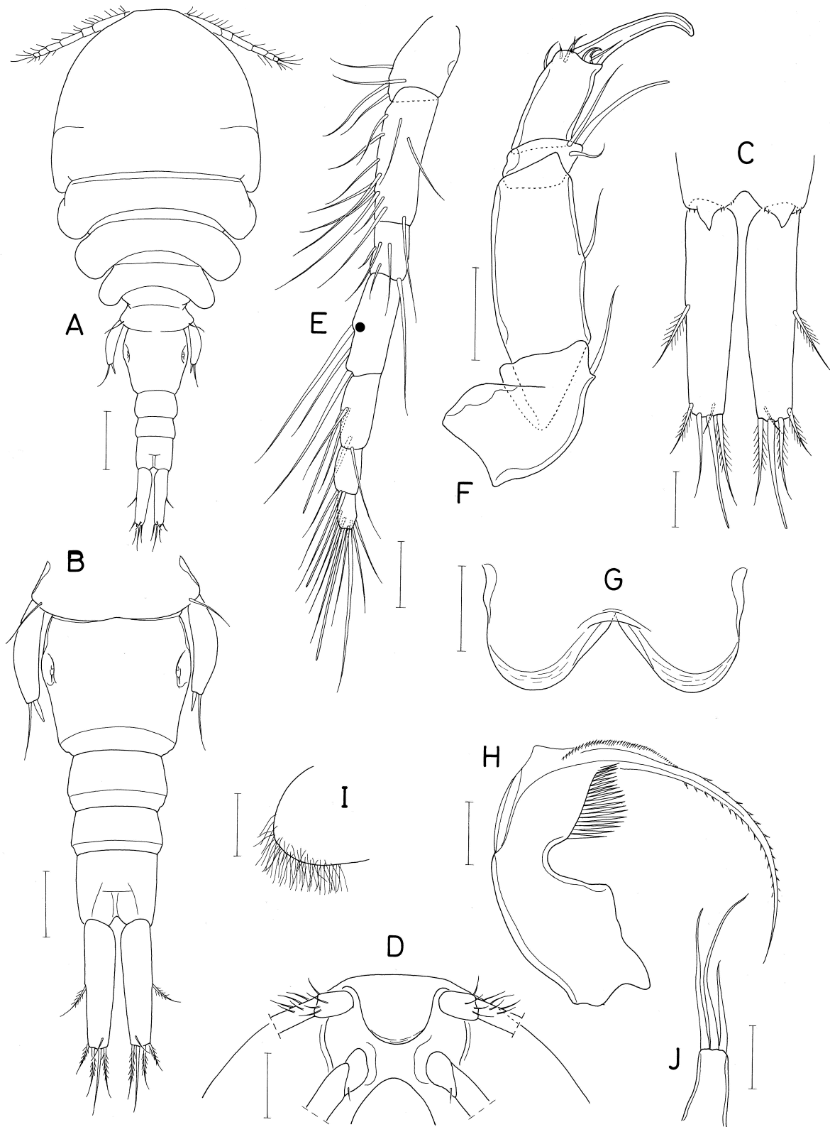
Fig. 53. Notoxynus lokobensis n. sp., female. A, habitus, dorsal; B, urosome, dorsal; C, caudal rami, ventral; D, rostral area, ventral; E, antennule (dot indicating place of additional aesthetasc in male); F, antenna; G, labrum; H, mandible; I, paragnath; J, maxillule. Scales: A, 0.2 mm; B, D, 0.1 mm; C, E-G, 0.05 mm; H-J, 0.02 mm.
