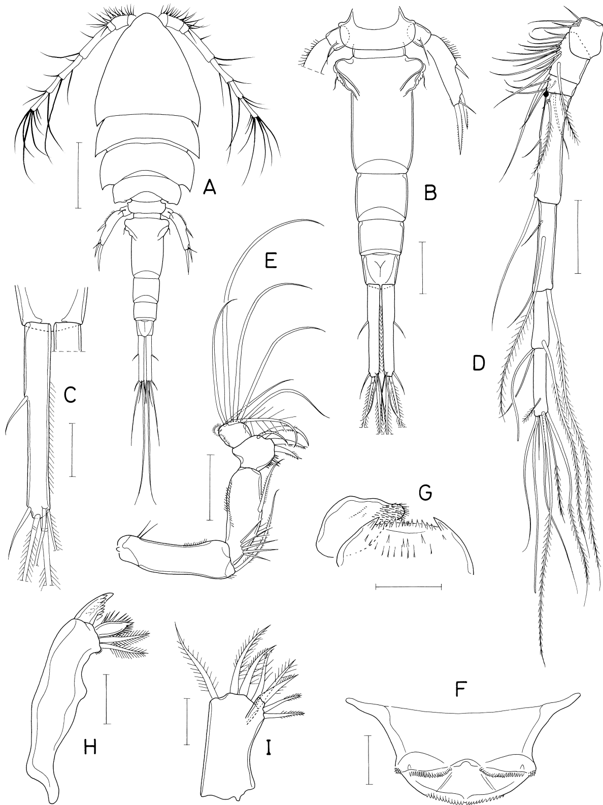
Fig. 7. Cemihyclops tenuis n. sp., female. A, habitus, dorsal; B, urosome, dorsal; C, caudal ramus, dorsal; D, antennule; E, antenna; F, labrum, dorsal; G, labium and right paragnath, ventral; H, mandible; I, maxillule. Scales: A, 0.5 mm; B, 0.2 mm; C-E, G, 0.1 mm; F, H, I, 0.05 mm.
