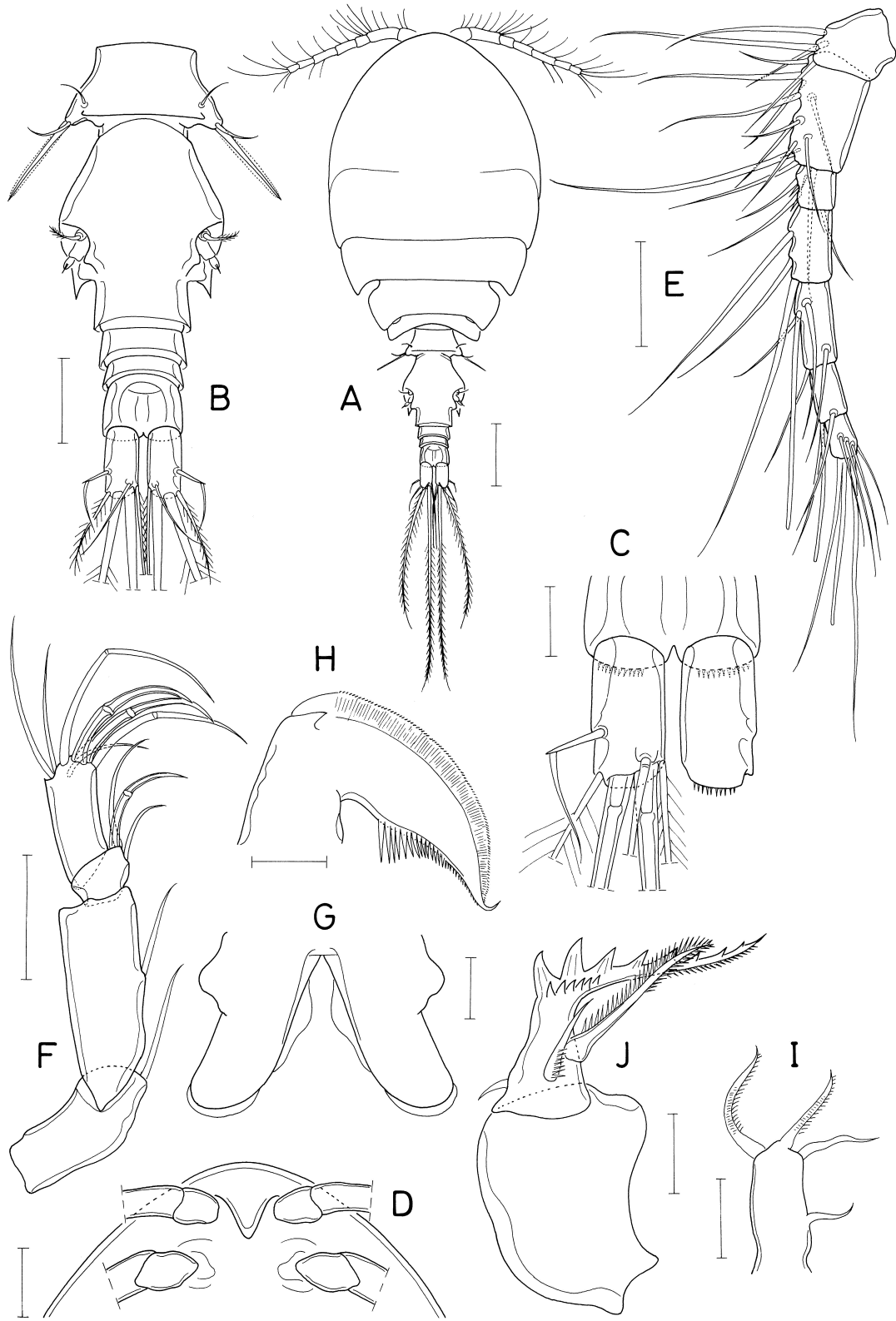
Fig. 44. Pseudanthessius acutus n. sp., female. A, habitus, dorsal; B, urosome, dorsal; C, caudal rami, dorsal; D, rostral area, ventral; E, antennule; F, antenna; G, labrum; H, mandible; I, maxillule; J, maxilla. Scales: A, 0.1 mm; B, D-F, 0.05 mm; C, G-J, 0.02 mm.
