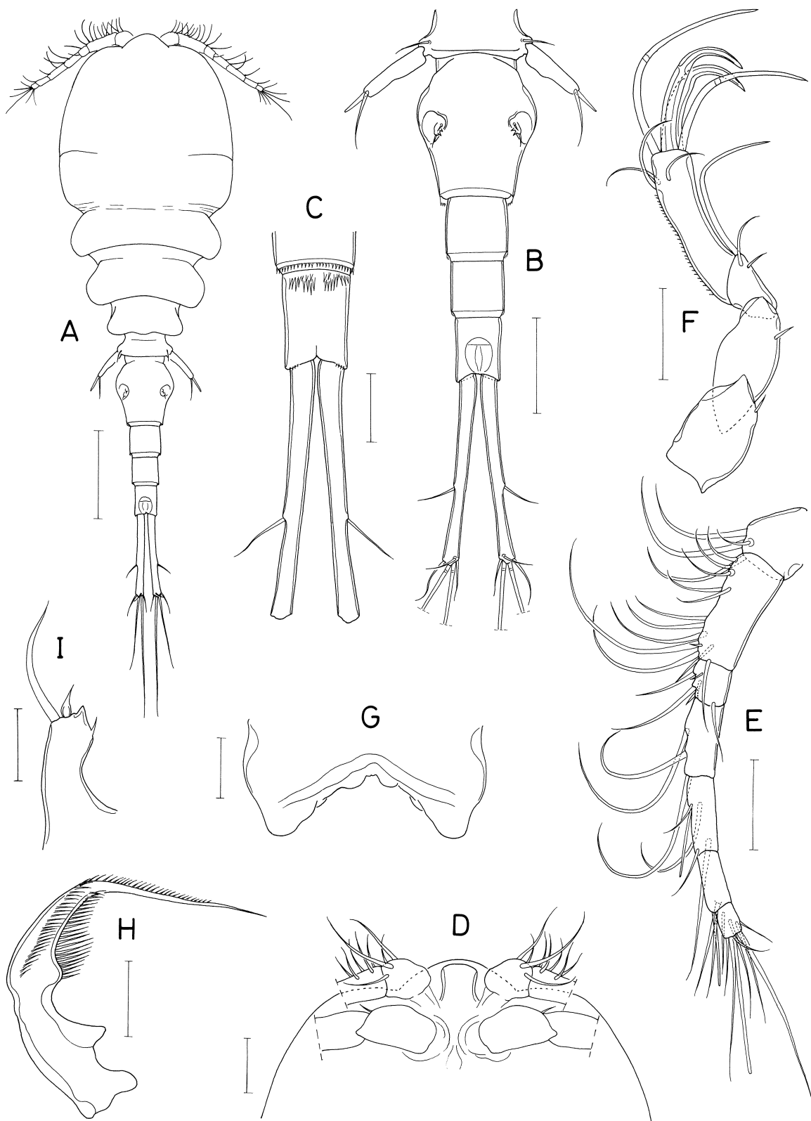
Fig. 35. Lichomolgus angustus n. sp., female. A, habitus, dorsal; B, urosome, dorsal; C, distal part of abdomen, ventral; D, rostral area, ventral; E, antennule; F, antenna; G, labrum; H, mandible; I, maxillule. Scales: A, 0.2 mm; B, 0.1 mm; C-F, 0.05 mm; G-I, 0.02 mm.
