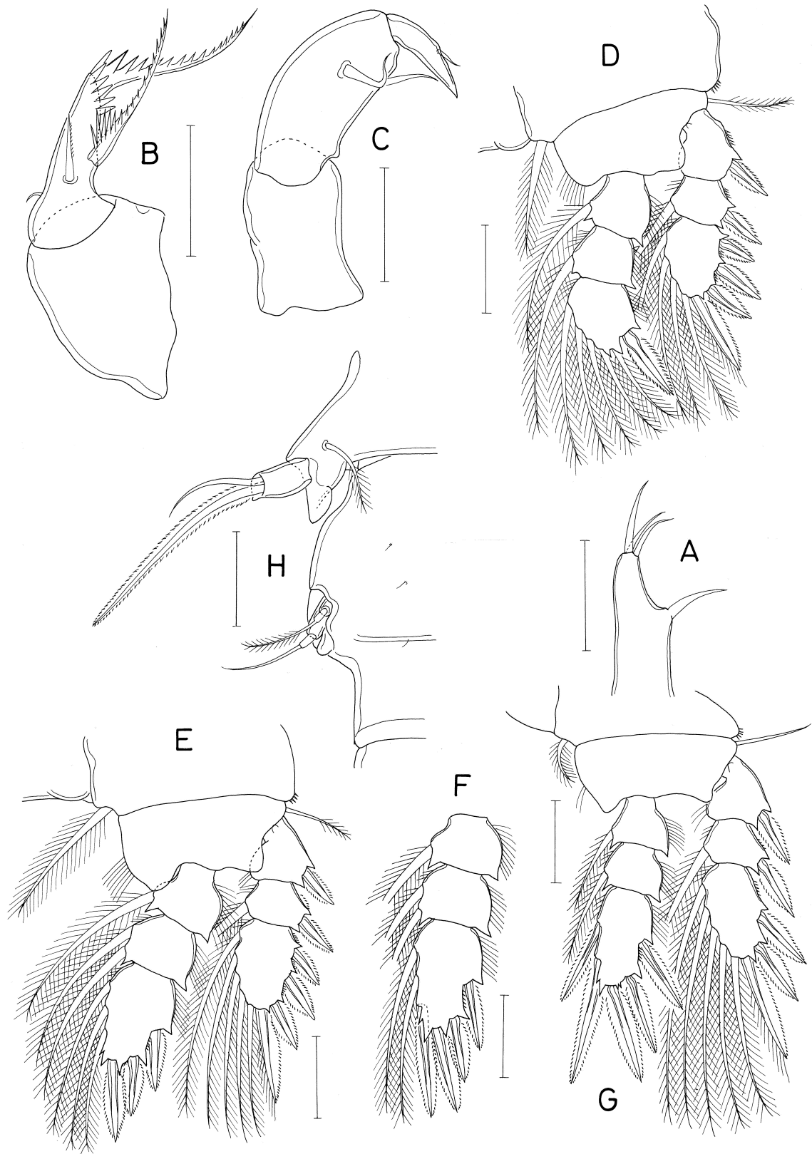
Fig. 59. Eupolymniphilus brevicaudatus n. sp., female. A, maxillule; B, maxilla; C, maxilliped; D, leg 1; E, leg 2; F, endopod of leg 3; G, leg 4; H, left side of first two urosomal somites, dorsal. Scales: 0.05 mm for all.
