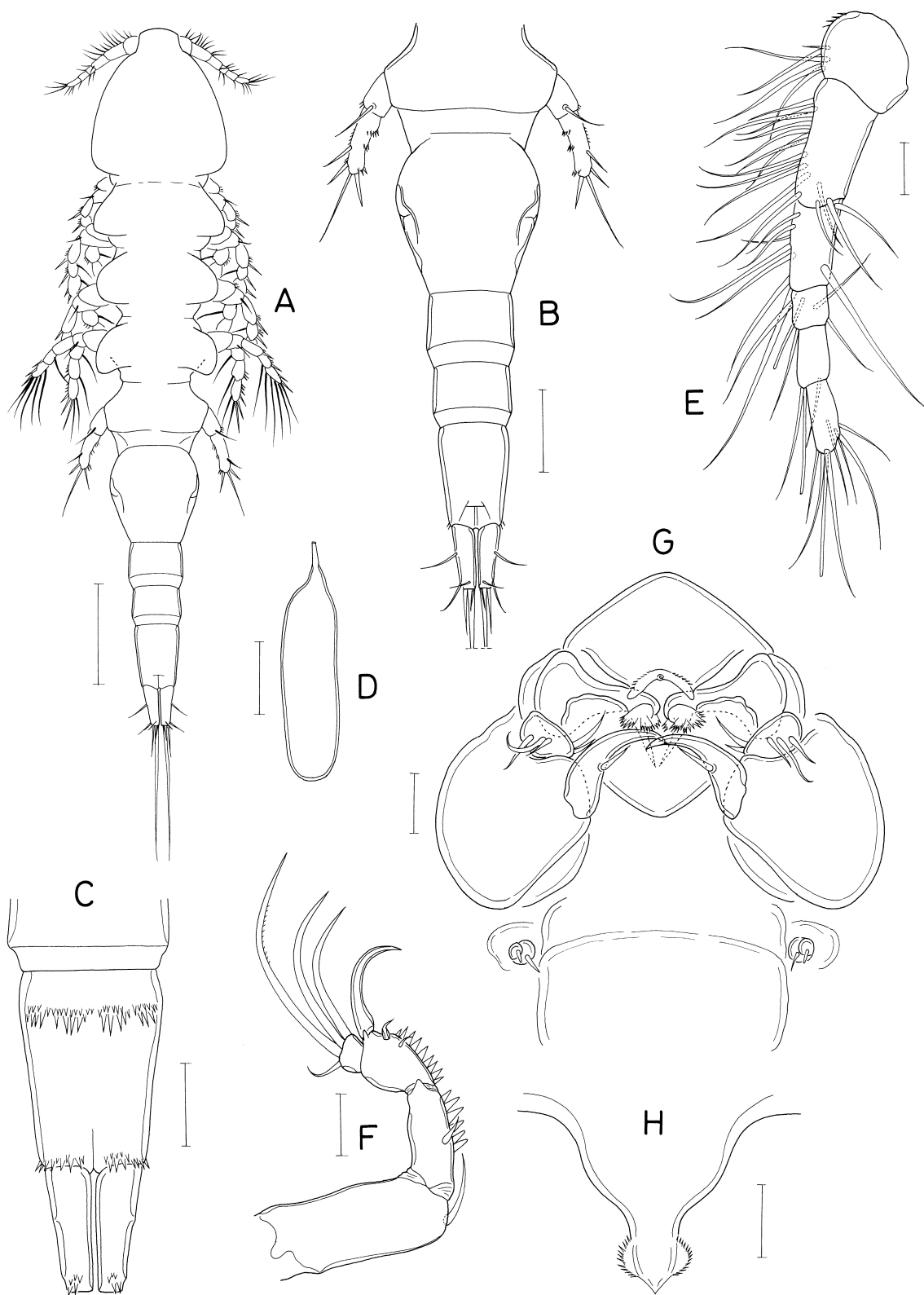
Fig. 23. Leptinogaster minutus n. sp., female. A, habitus, dorsal; B, urosome, dorsal; C, distal part of abdomen, ventral; D, spermatophore from female; E, antennule; F, antenna; G, oral area; H, labrum. Scales: A, 0.2 mm; B, 0.1 mm; C, D, 0.05 mm; E-H, 0.02 mm.
