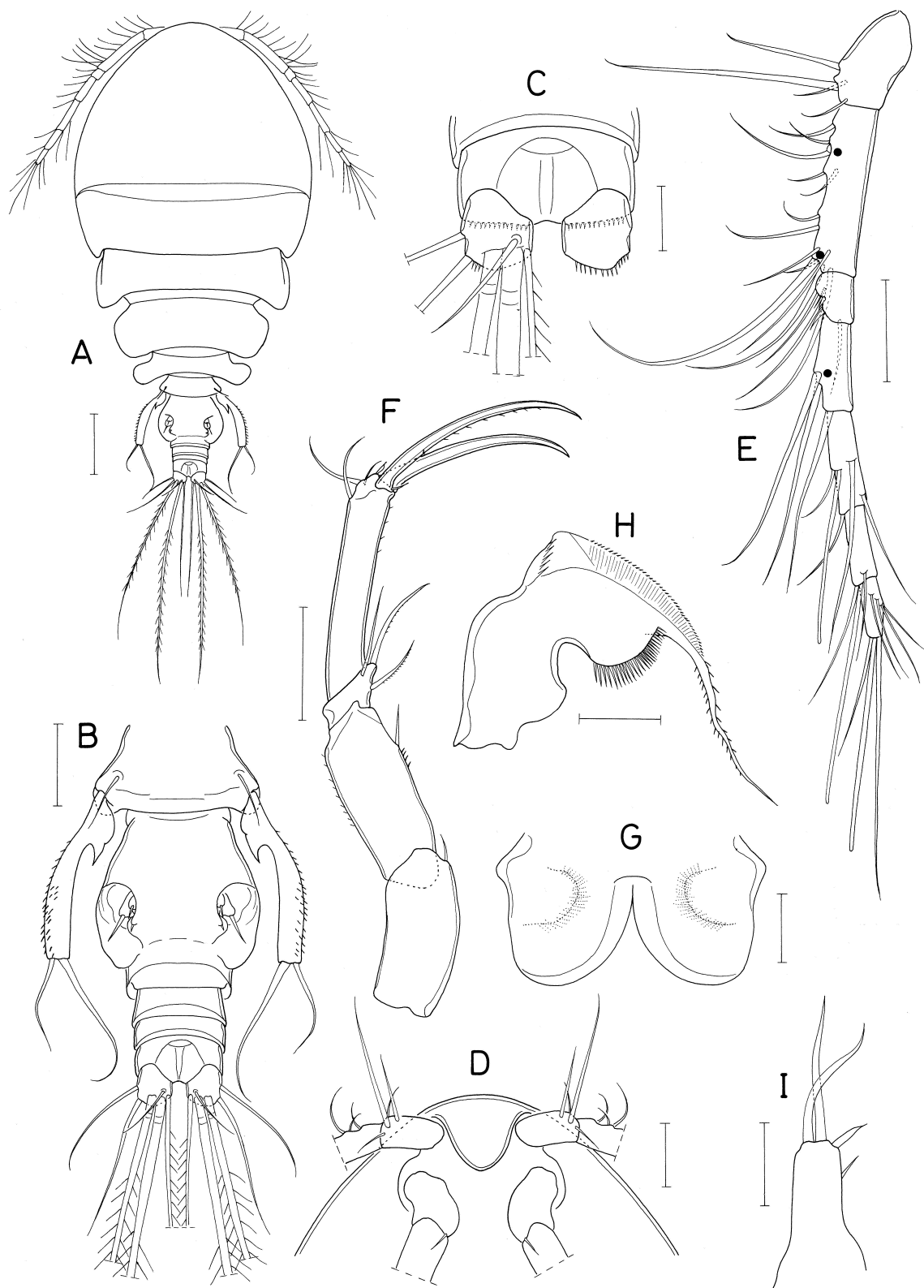
Fig. 50. Acanthomolgus tenuispinatus n. sp., female. A, habitus, dorsal; B, urosome, dorsal; C, anal somite and caudal rami, dorsal; D, rostral area, ventral; E, antennule (dots indicating places of additional aesthetascs in male); F, antenna; G, labrum; H, mandible; I, maxillule. Scales: A, 0.1 mm; B, D-F, 0.05 mm; C, G-I, 0.02 mm.
