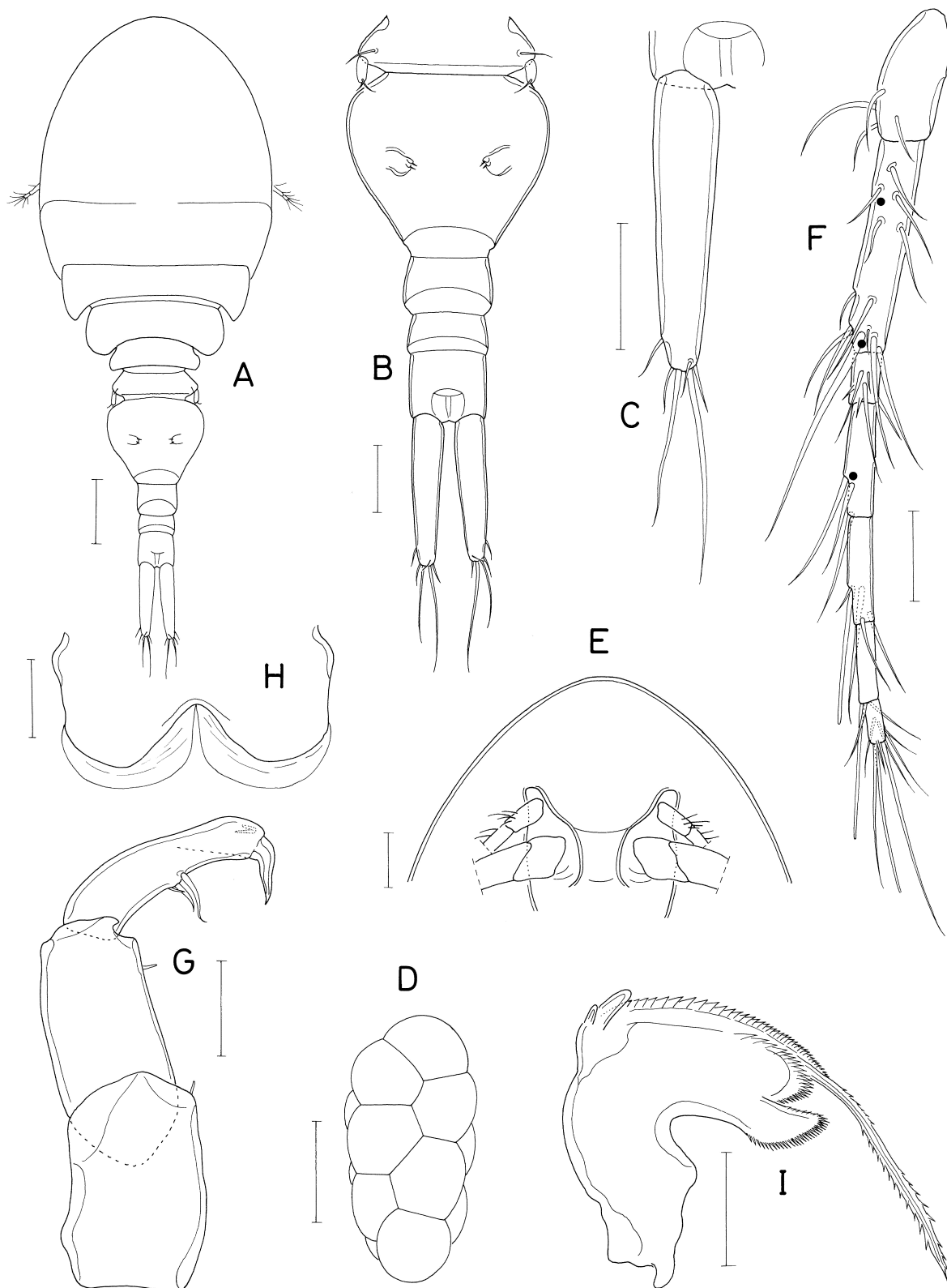
Fig. 29. Schedomolgus parvipediger n. sp., female. A, habitus, dorsal; B, urosome, dorsal; C, left caudal ramus, dorsal; D, egg sac; E, rostral area, ventral; F, antennule (dots indicating places of additional aesthetascs in male); G, antenna; H, labrum; I, mandible. Scales: A, D, 0.2 mm; B, C, E, 0.1 mm; F-I, 0.05 mm.
