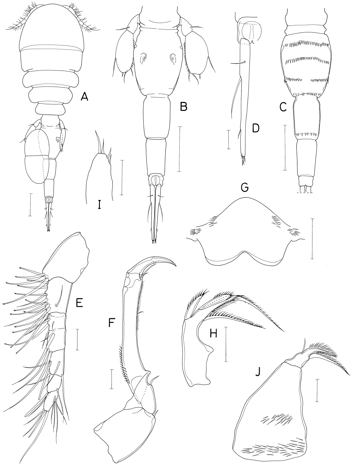
Fig. 64. Ostrincola binoviger n. sp., female. A, habitus, dorsal; B, urosome, dorsal; C, urosome, ventral; D, left caudal ramus, dorsal; E, antennule; F, antenna; G, labrum; H, mandible; I, maxillule; J, maxilla. Scales: A-C, 0.1 mm; D-F, H-J, 0.02 mm; G, 0.05 mm.
