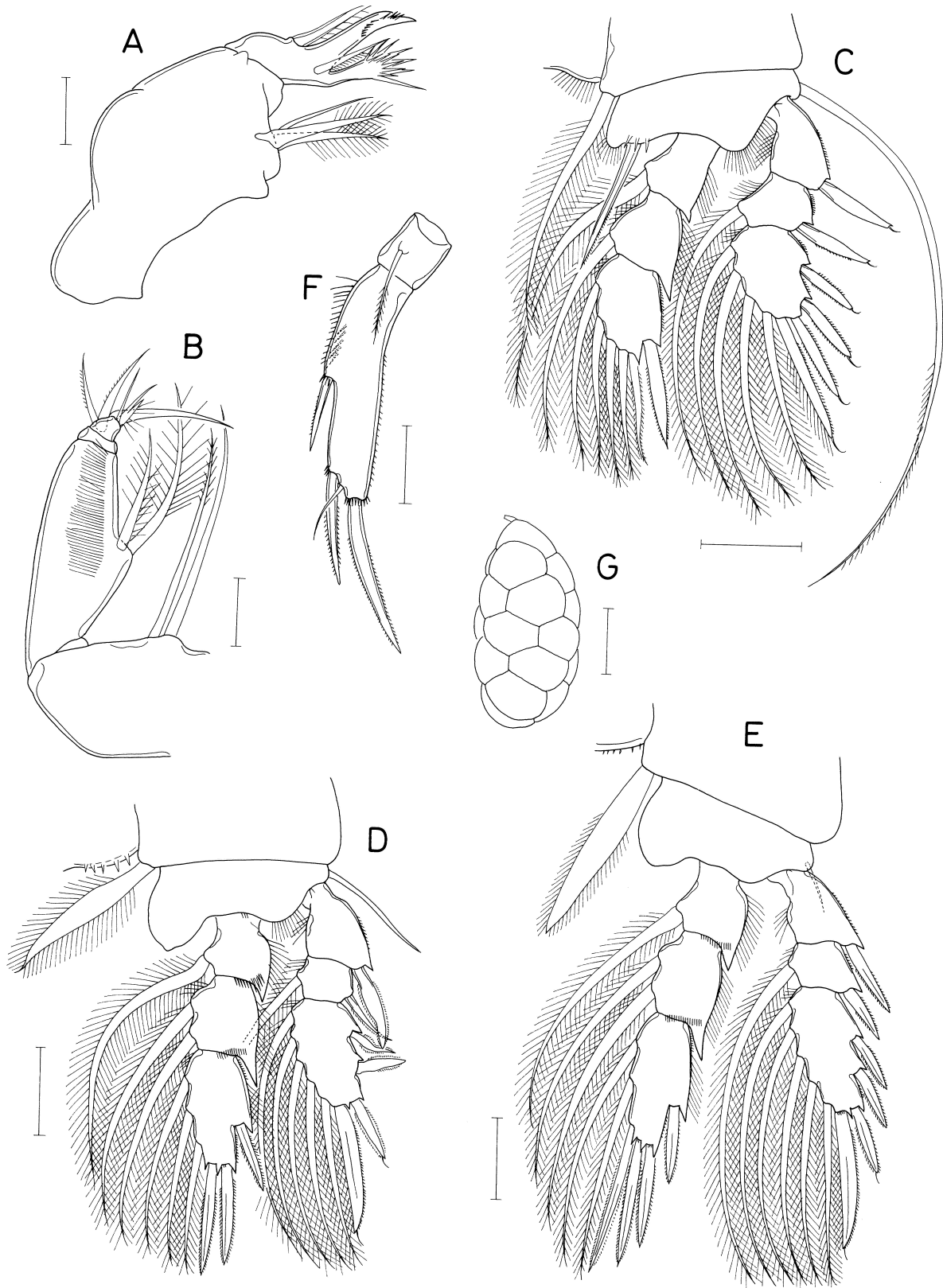
Fig. 8. Cemihyclops tenuis n. sp., female. A, maxilla; B, maxilliped; C, leg 1; D, leg 2; E, leg 3; F, leg 5; G, egg sac. Scales: A, B, 0.05 mm; C-F, 0.1 mm; G, 0.2 mm.
