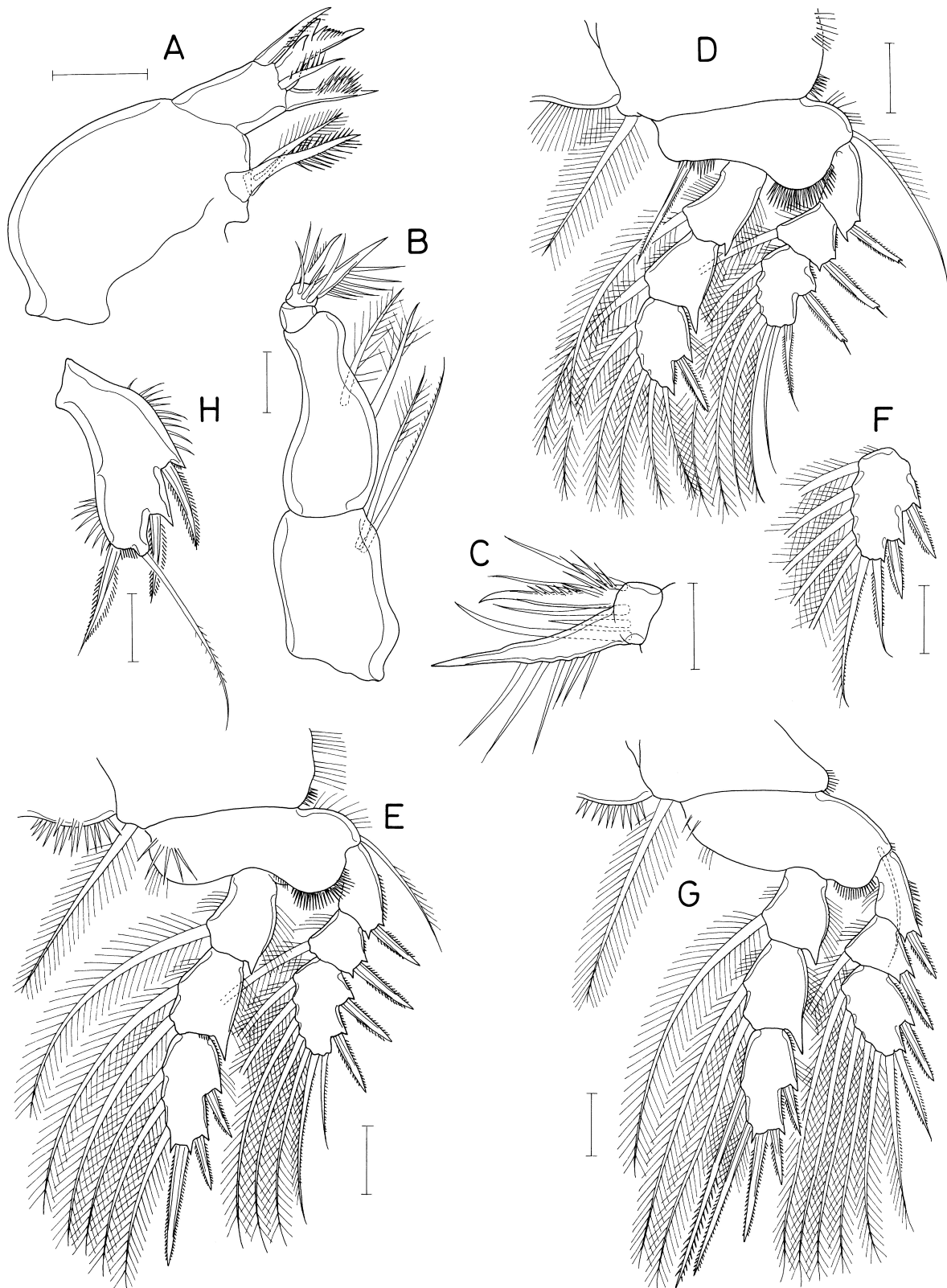
Fig. 18. Hemicyclops humesi n. sp., female. A, maxilla; B, maxilliped; C, distal part of maxilliped; D, leg 1; E, leg 2; F, third exopodal segment of leg 3; G, leg 4; H, free segment of leg 5. Scales: A, D-H, 0.05 mm; B, C, 0.02 mm.
