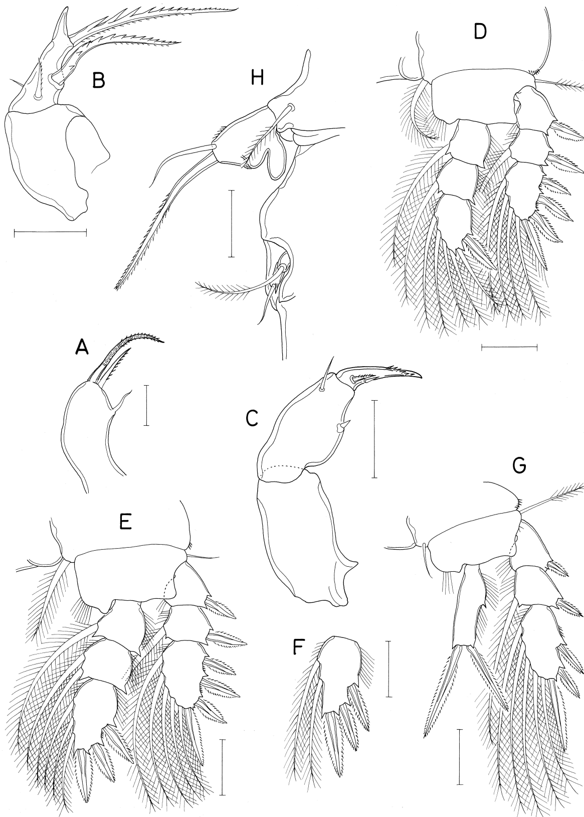
Fig. 49. Tubiporicola inflatus n. sp., female. A, maxillule; B, maxilla; C, maxilliped; D, leg 1; E, leg 2; F, third endopodal segment of leg 3; G, leg 4; H, left side of first two urosomal somites, dorsal. Scales: A, 0.02 mm; B-H, 0.05 mm.
