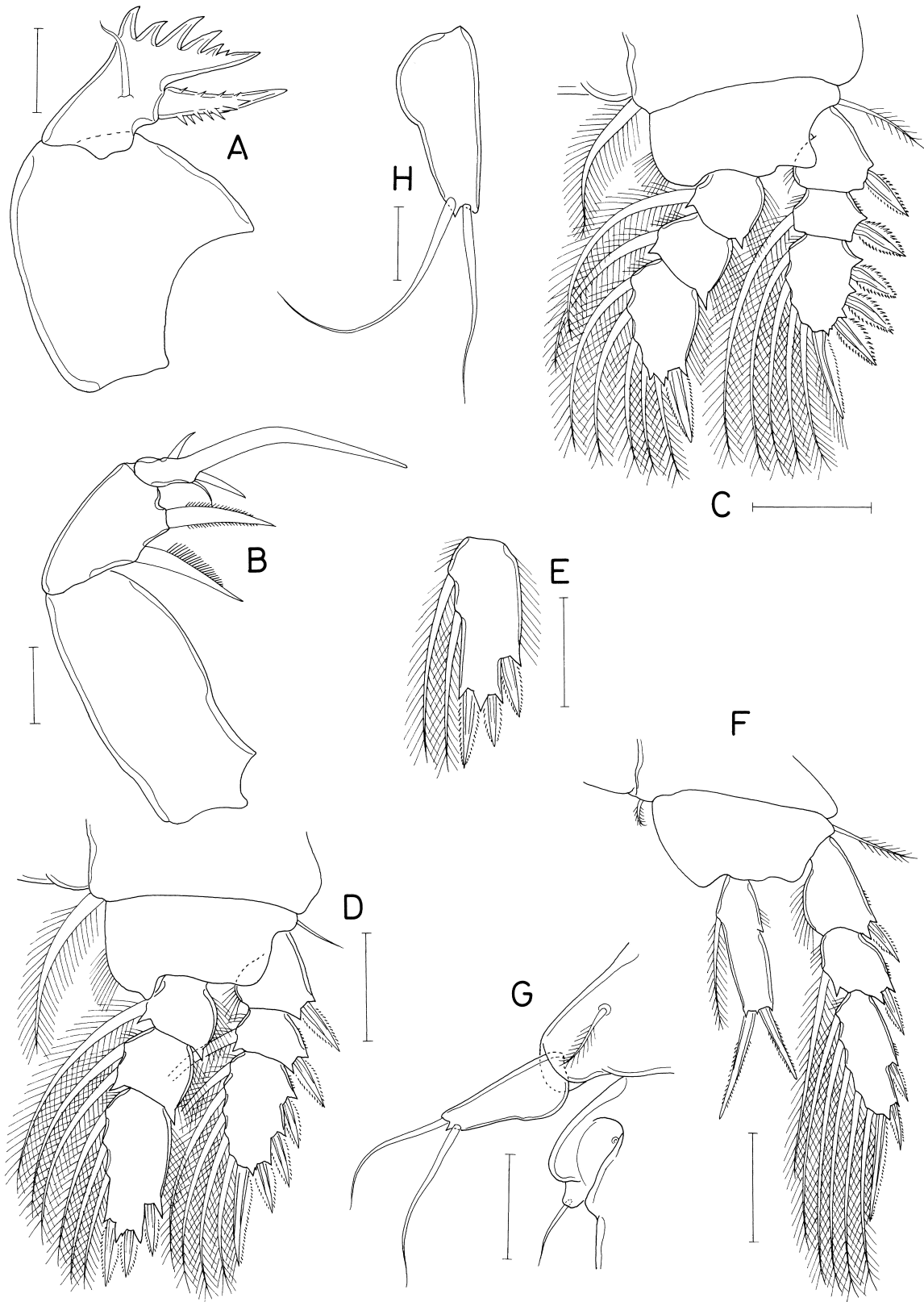
Fig. 33. Kellera multiovigera n. sp., female. A, maxilla; B, maxilliped; C, leg 1; D, leg 2; E, third endopodal segment of leg 3; F, leg 4; G, left side of first two urosomal somites, dorsal; H, free segment of leg 5. Scales: A, B, H, 0.05 mm; C-G, 0.1 mm.
