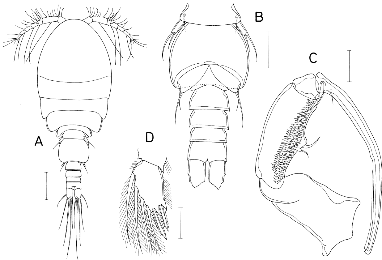
Fig. 34. Kellieria multiovigera n. sp., male. A, habitus, dorsal; B, urosome, ventral; C, maxilliped; D, third endopodal segment of leg 1. Scales: A, 0.2 mm; B, 0.1 mm; C, D, 0.05 mm.
