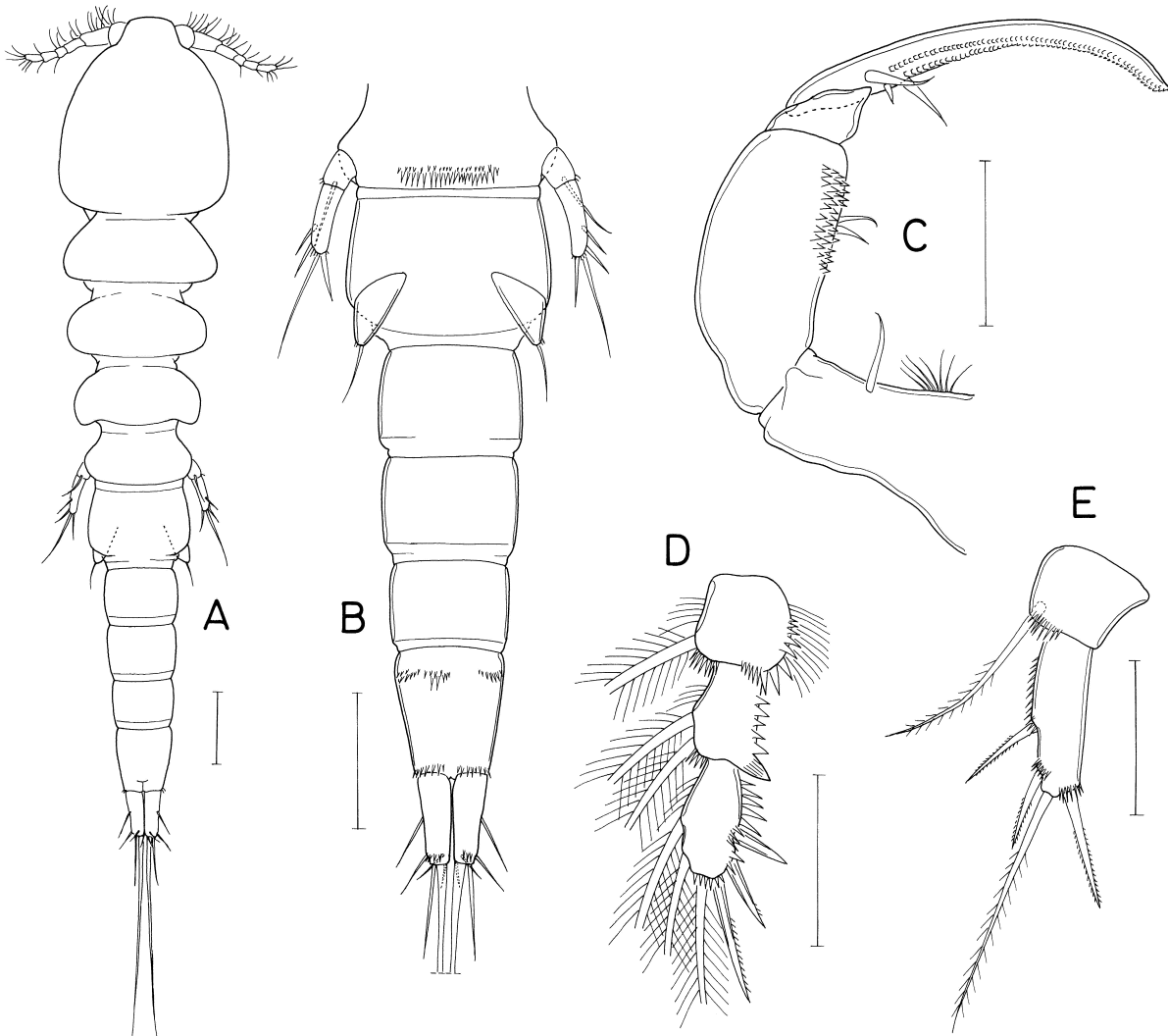
Fig. 25. Leptinogaster minuta n. sp., male. A, habitus, dorsal; B, urosome, ventral; C, maxilliped; D, endopod of leg 2; E, leg 5. Scales: A, B, 0.1 mm; C-E, 0.05 mm.
