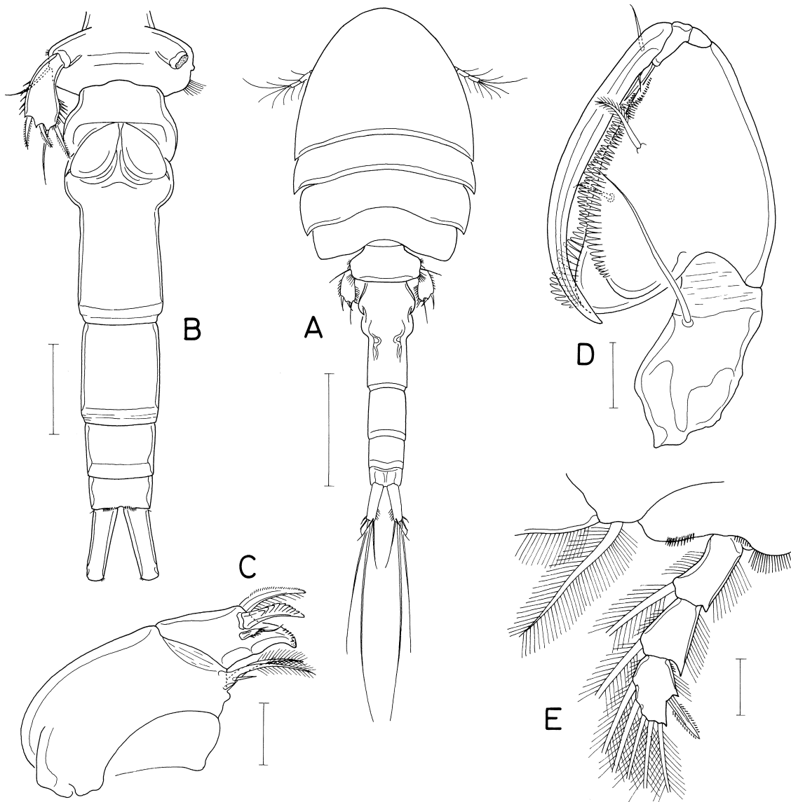
Fig. 16. Hemicyclops tripartitus n. sp., male. A, habitus, dorsal; B, urosome, ventral; C, maxilla; D, maxilliped; E, endopod of leg 1. Scales: A, 0.5 mm; B, 0.2 mm; C-E, 0.05 mm.
