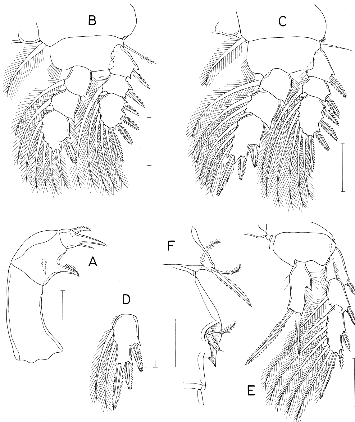
Fig. 45. Pseudanthessius acutus n. sp., female. A, maxilliped; B, leg 1; C, leg 2; D, third endopodal segment of leg 3; E, leg 4; F, right side of first two urosomal somites, dorsal. Scales: A, 0.02 mm; B-F, 0.05 mm.
