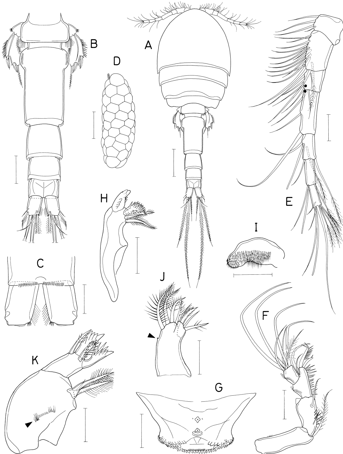
Fig. 10. Hemicyclops columnaris Humes, female. A, habitus, dorsal; B, urosome, dorsal; C, caudal rami, ventral; D, egg sac; E, antennule; F, antenna; G, labrum, dorsal; H, mandible; I, paragnath; J, maxillule; K, maxilla. Scales: A, 0.2 mm; B, D, 0.1 mm; C, E-K, 0.05 mm.
