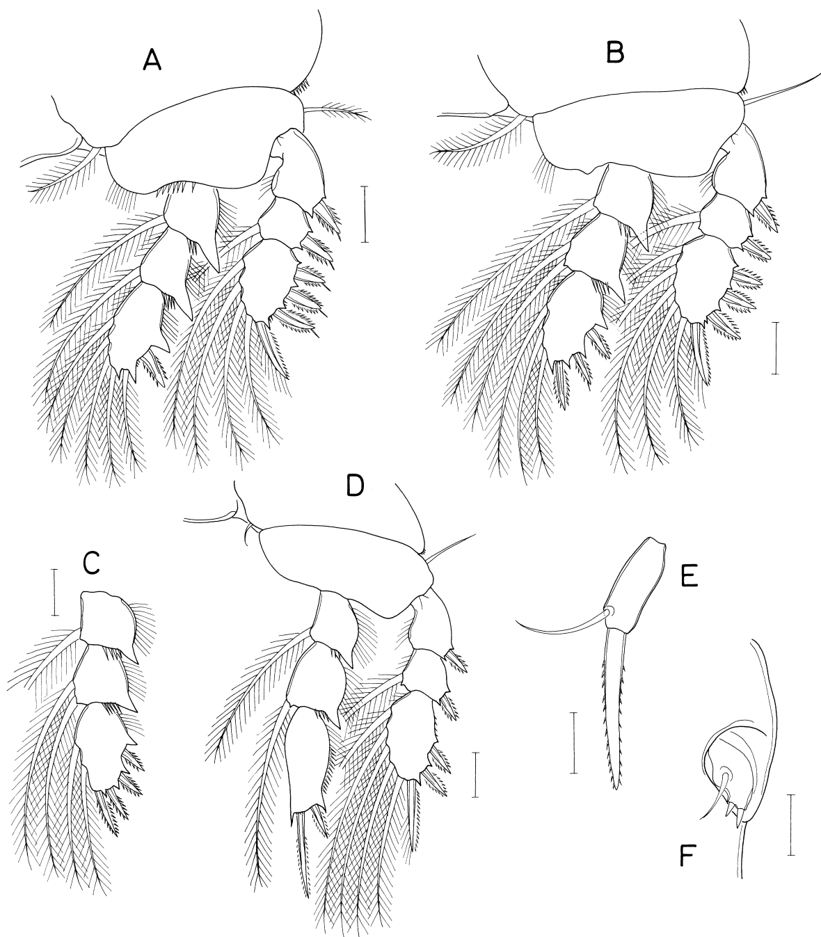
Fig. 42. Modiolicola trabalis Humes, female. A, leg 1; B, leg 2; C, endopod of leg 3; D, leg 4; E, free segment of leg 5; F, right genital area. Scales: 1.02 mm for all.
