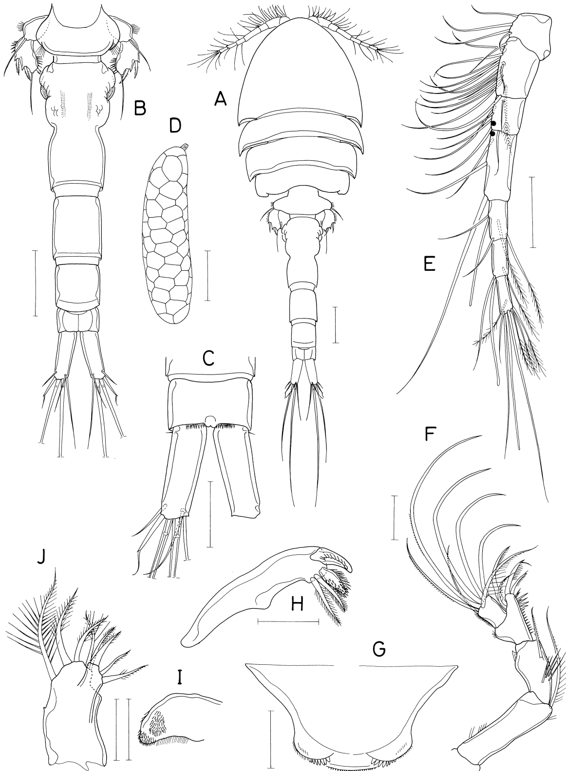
Fig. 17. Hemicyclops humesi n. sp., female. A, habitus, dorsal; B, urosome, dorsal; C, anal somite and caudal rami, ventral; D, egg sac; E, antennule; F, antenna; G, labrum, dorsal; H, mandible; I, paragnath; J, maxillule. Scales: A, B, D, 0.1 mm; C, E, 0.1 mm; F-J, 0.05 mm.
