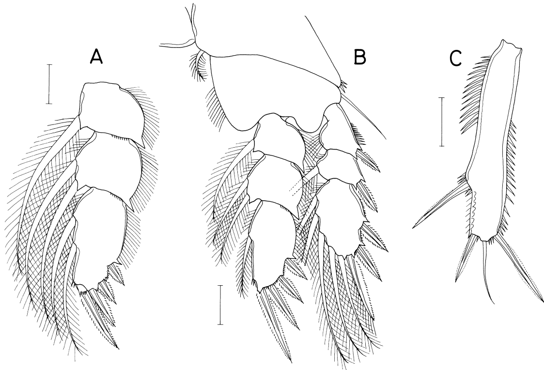
Fig. 6. Discanthessus solitarius n. gen. n. sp., female. A, endopod of leg 3; B, leg 4; C, free segment of leg 5. Scales: 0.05 mm for all.
