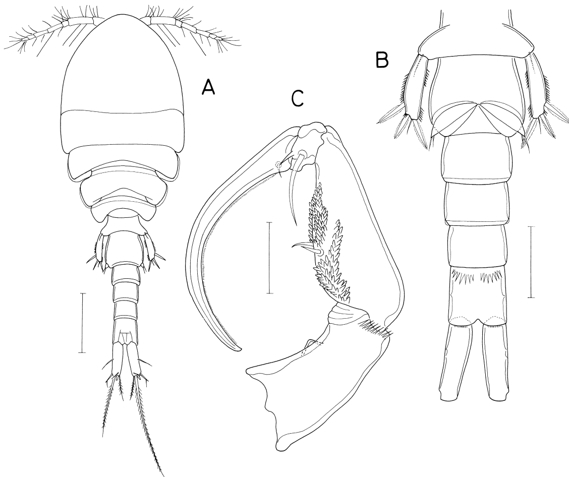
Fig. 3. Anthessius nosybensis n. sp., male. A, habitus, dorsal; B, urosome, ventral; C, maxilliped. Scales: A, 0.2 mm; B, 0.1 mm; C, 0.05 mm.
