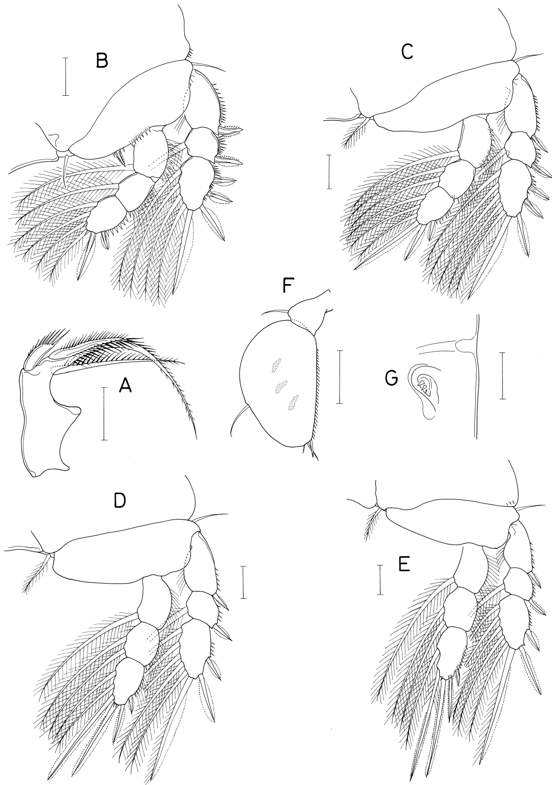
Fig. 63. Ostrincola breviseti Ho and Kim, female. A, mandible; B, leg 1; C, leg 2; D, leg 3; E, leg 4; F, leg 5; G, right genital area. Scales: A-E, G, 0.02 mm; F, 0.05 mm.
