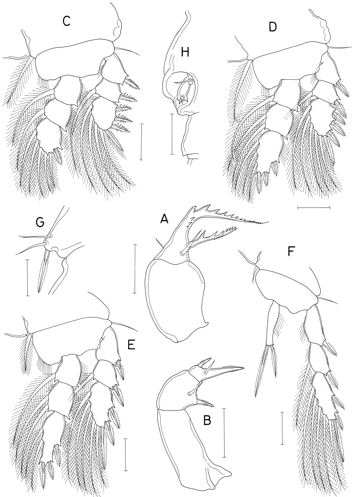
Fig. 47. Pseudanthessius asper n. sp., female. A, maxilla; B, maxilliped; C, leg 1; D, leg 2; E, leg 3; F, leg 4; G, leg 5; H, left genital area. Scales: 0.05 mm for all.
