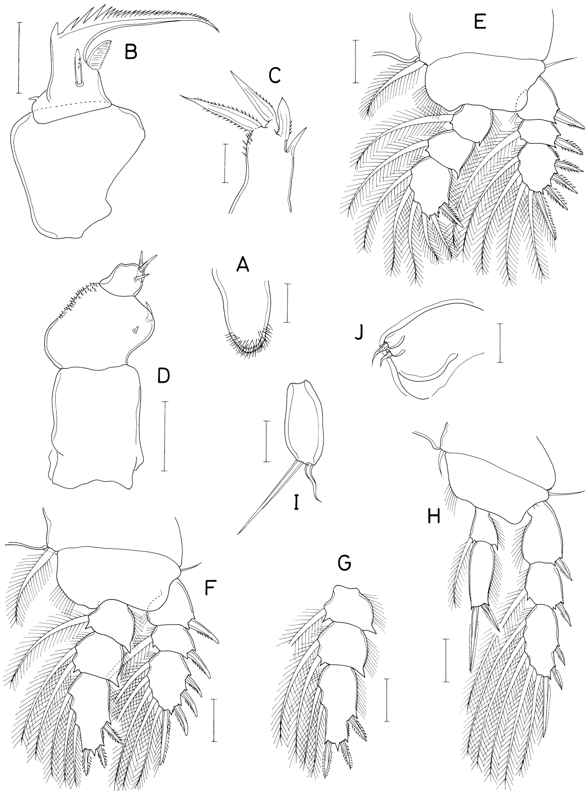
Fig. 30. Schedomolgus parvipediger n. sp., female. A, paragnath; B, maxilla; C, maxillule; D, maxilliped; E, leg 1; F, leg 2; G, endopod of leg 3; H, leg 4; I, free segment of 5; J, right genital area. Scales: A, C, I, J, 0.02 mm; B, D-H, 0.05 mm.
