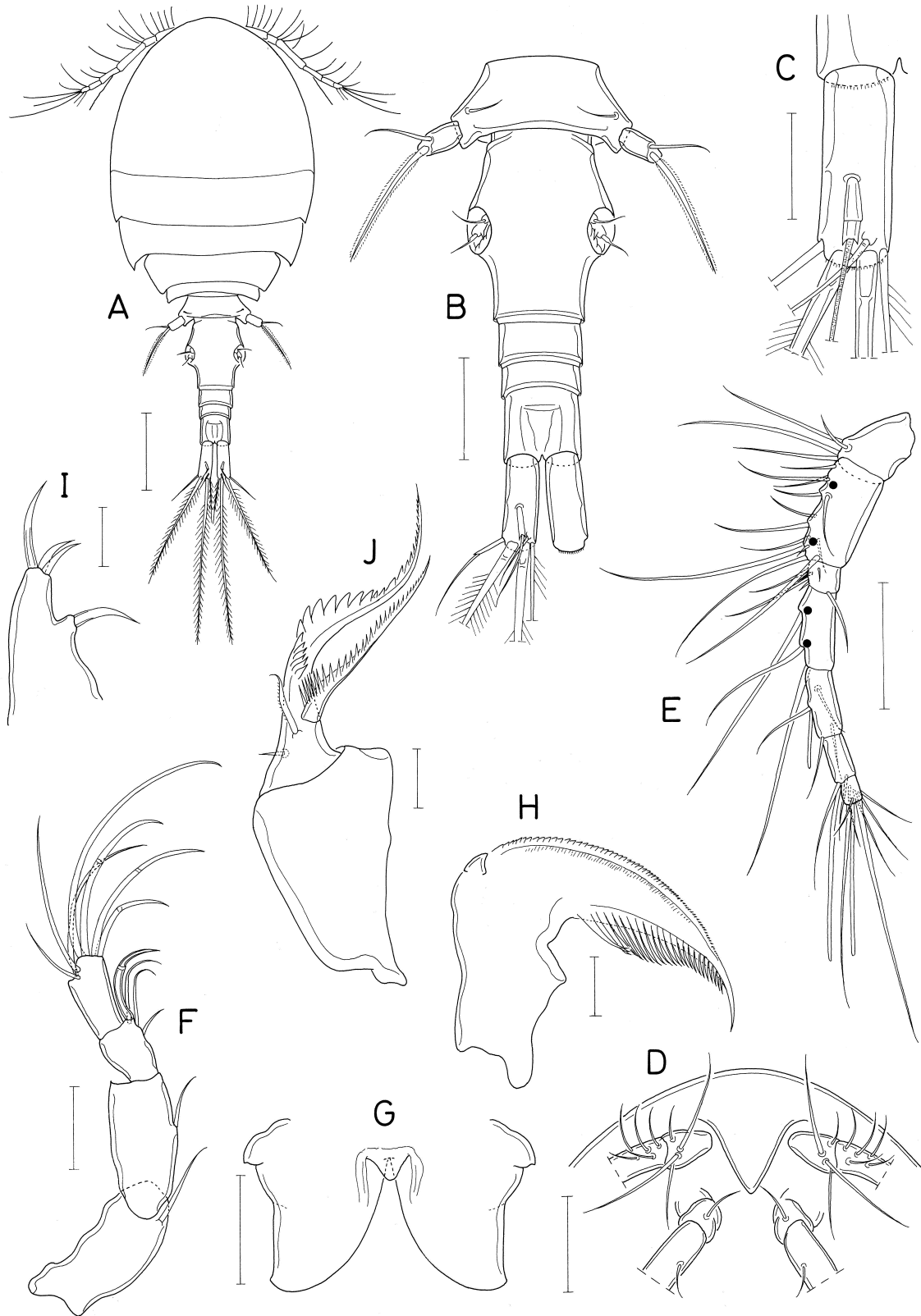
Fig. 56. Eupolymniphilus occidentalis n. sp., female. A, habitus, dorsal; B, urosome, dorsal; C, left caudal ramus, dorsal; D, rostral area, ventral; E, antennule (dots indicating places of additional aesthetascs in male); F, antenna; G, labrum; H, mandible; I, maxillule; J, maxilla. Scales: A, 0.2 mm; B, D, E, 0.1 mm; C, F, G, 0.05 mm; H-J, 0.02 mm.
