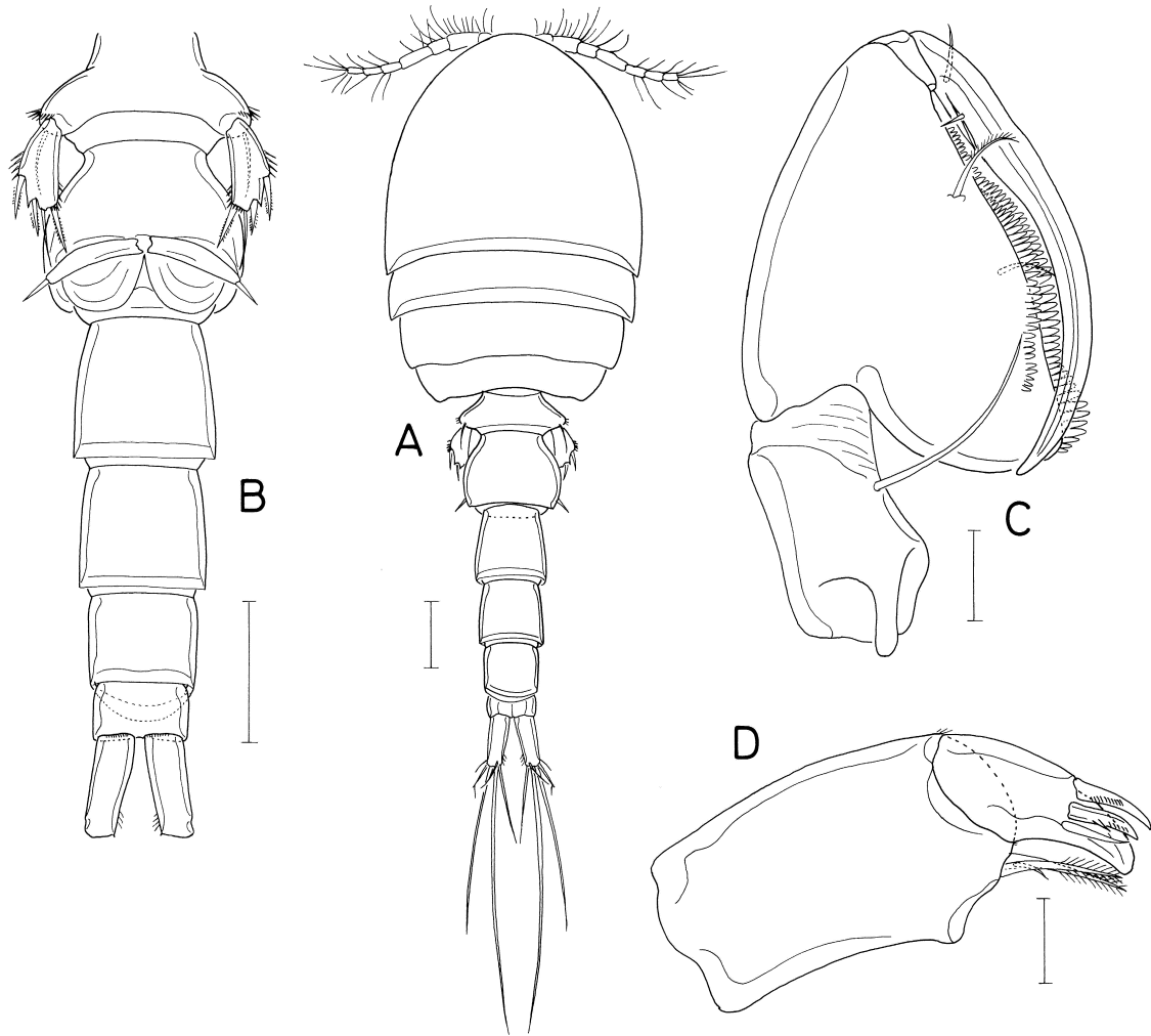
Fig. 19. Hemicyclops humesi n. sp., male. A, habitus, dorsal; B, urosome, ventral; C, maxilliped; D, maxilla. Scales: A, B, 0.2 mm; C, D, 0.05 mm.
