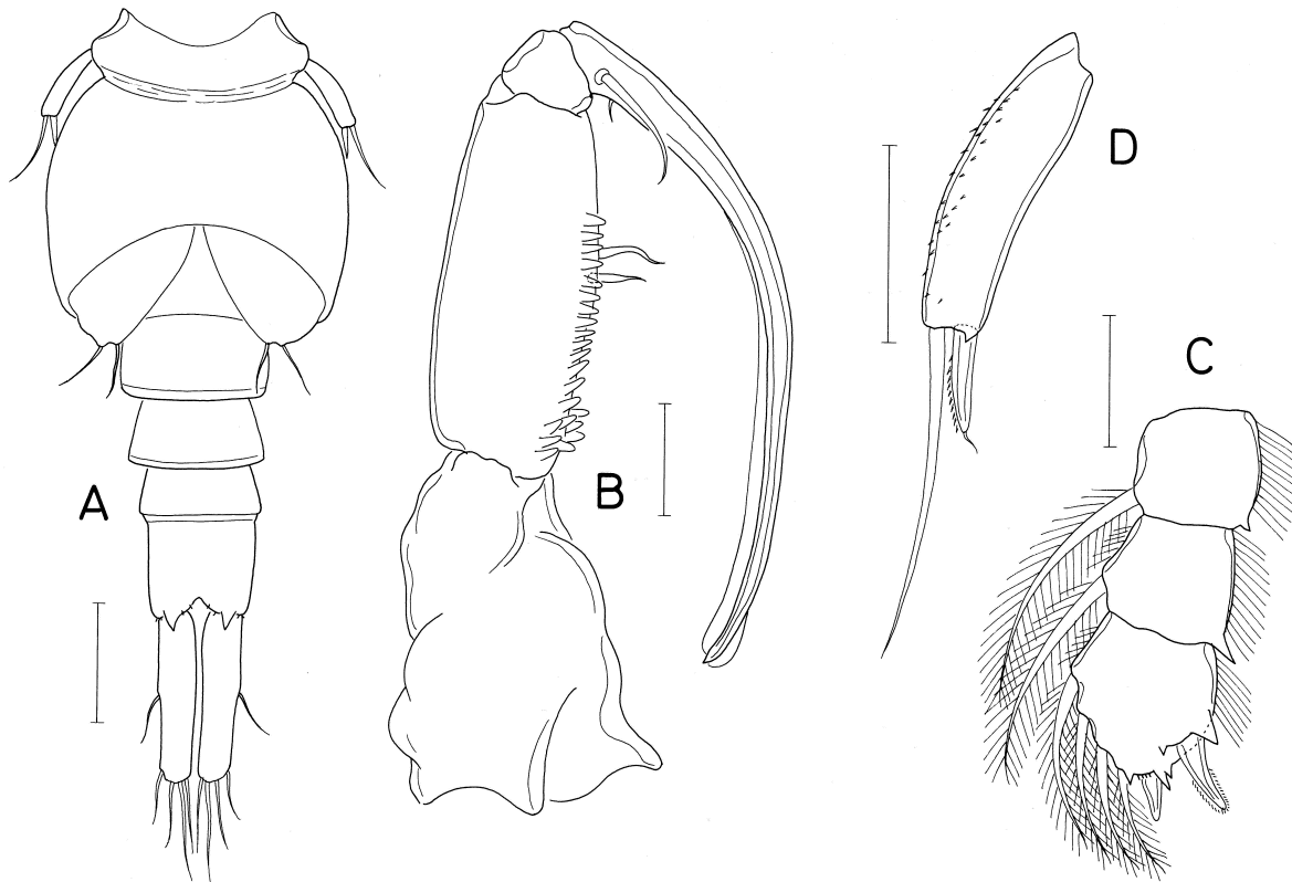
Fig. 55. Notoxynus lokobensis n. sp., male. A, urosome, ventral; B, maxilliped; C, endopod of leg 1; D, free segment of leg 5. Scales: A, 0.1 mm; B-D, 0.05 mm.
