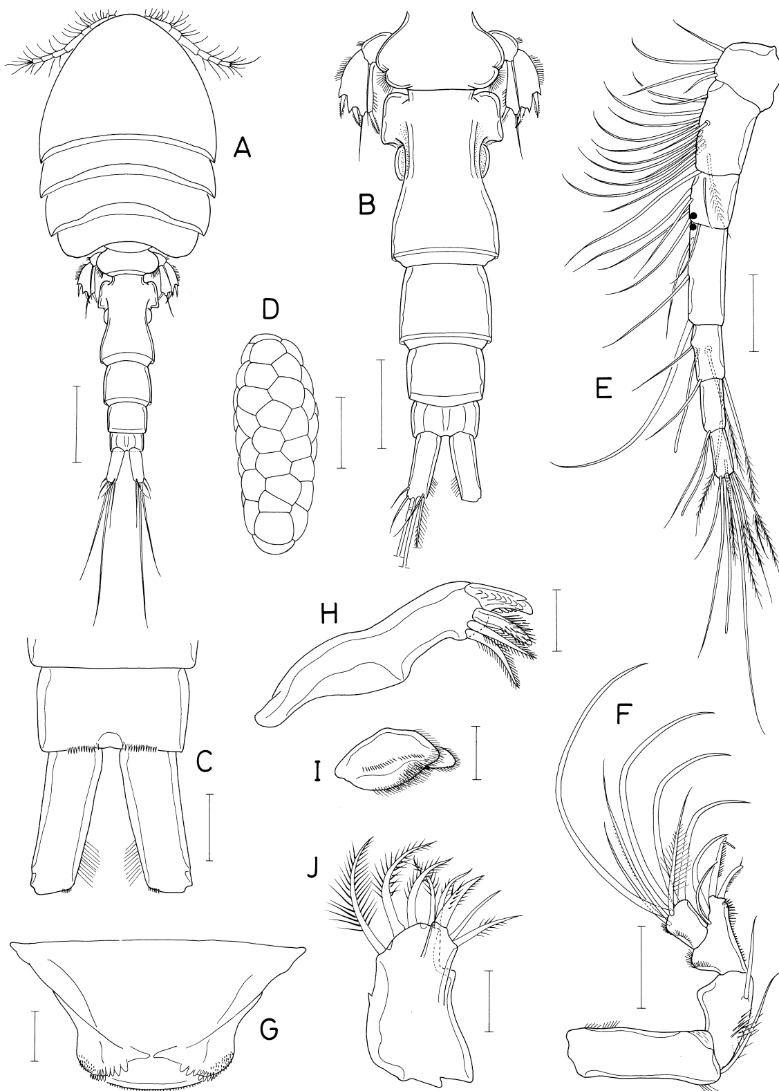
Fig. 20. Hemicyclops magnus n. sp., female. A, habitus, dorsal; B, urosome, dorsal; C, anal somite and caudal rami, ventral; D, egg sac; E, antennule; F, antenna; G, labrum, dorsal; H, mandible; I, paragnath; J, maxillule. Scales: A, 0.5 mm; B, D, 0.2 mm; C, E, F, 0.1 mm; G-J, 0.05 mm.
