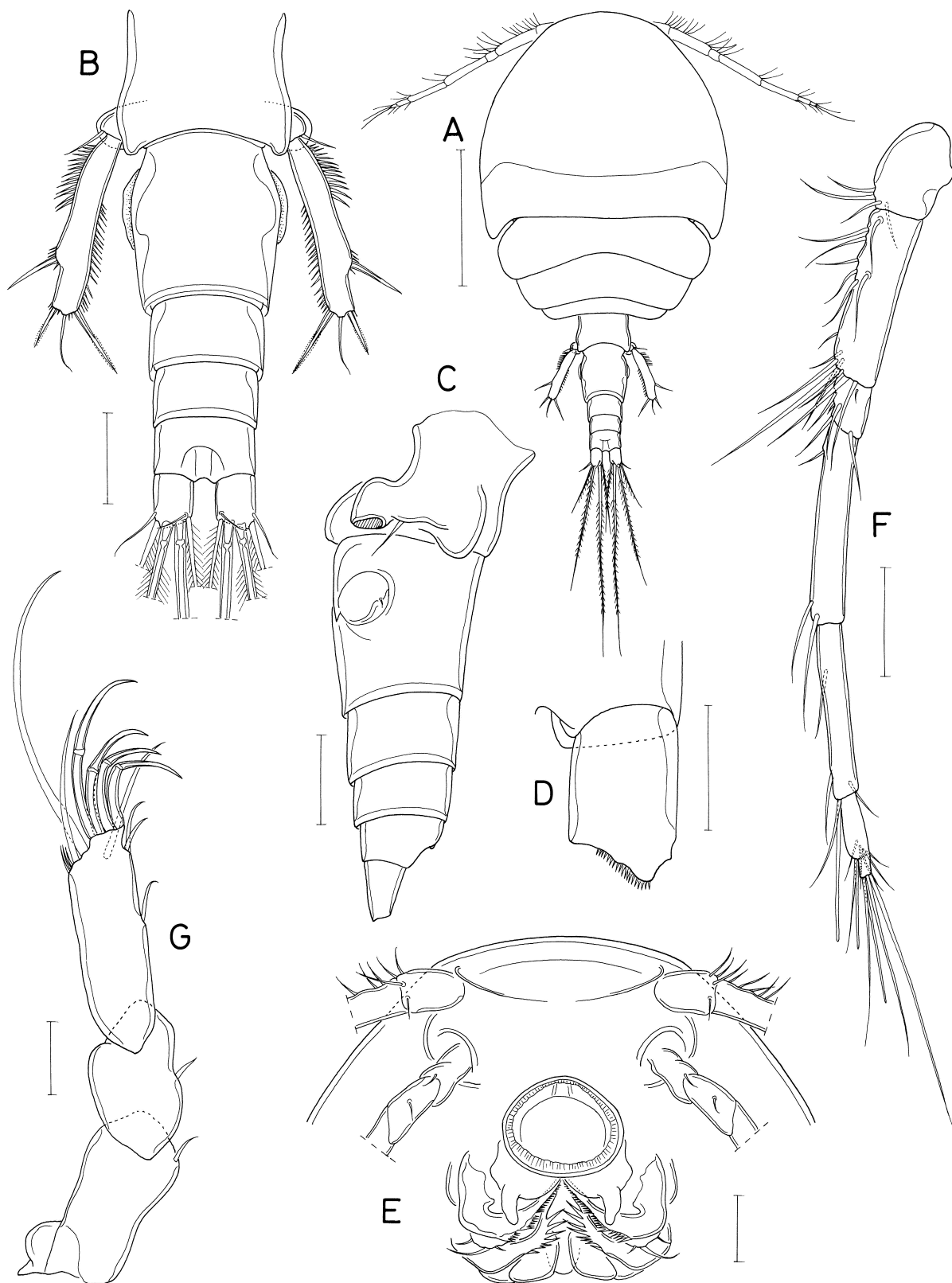
Fig. 4. Discanthessus solitarius n. gen. n. sp., female. A, habitus, dorsal; B, urosome, dorsal; C, urosome, lateral; D, left caudal ramus, ventral; E, cephalic area, ventral; F, antennule; G, antenna. Scales: A, 0.5 mm; B, C, E, F, 0.1 mm; D, G, 0.05 mm.
