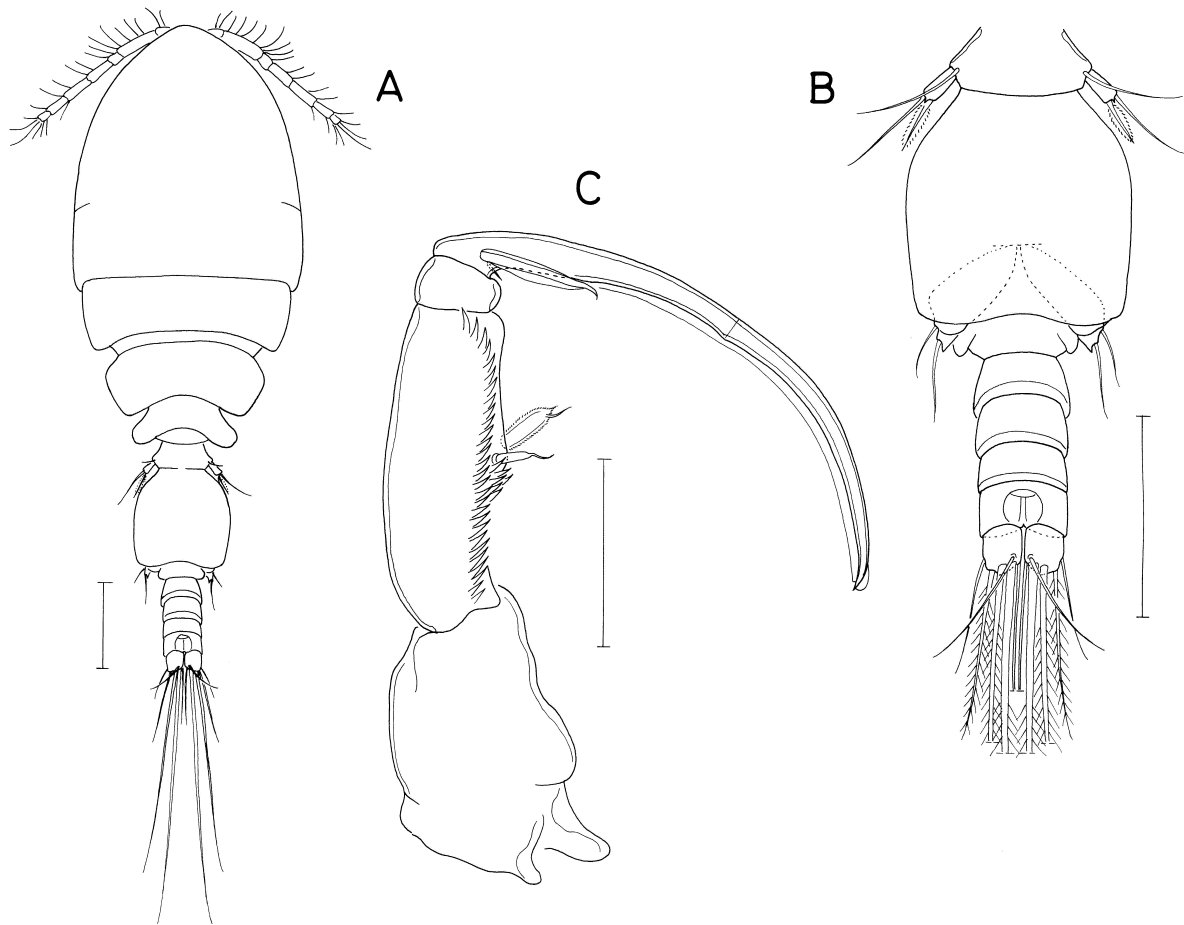
Fig. 40. Lichomolgus fusiformis n. sp., male. A, habitus, dorsal; B, urosome, dorsal; C, maxilliped. Scales: A, B, 0.1 mm; C, 0.05 mm.
