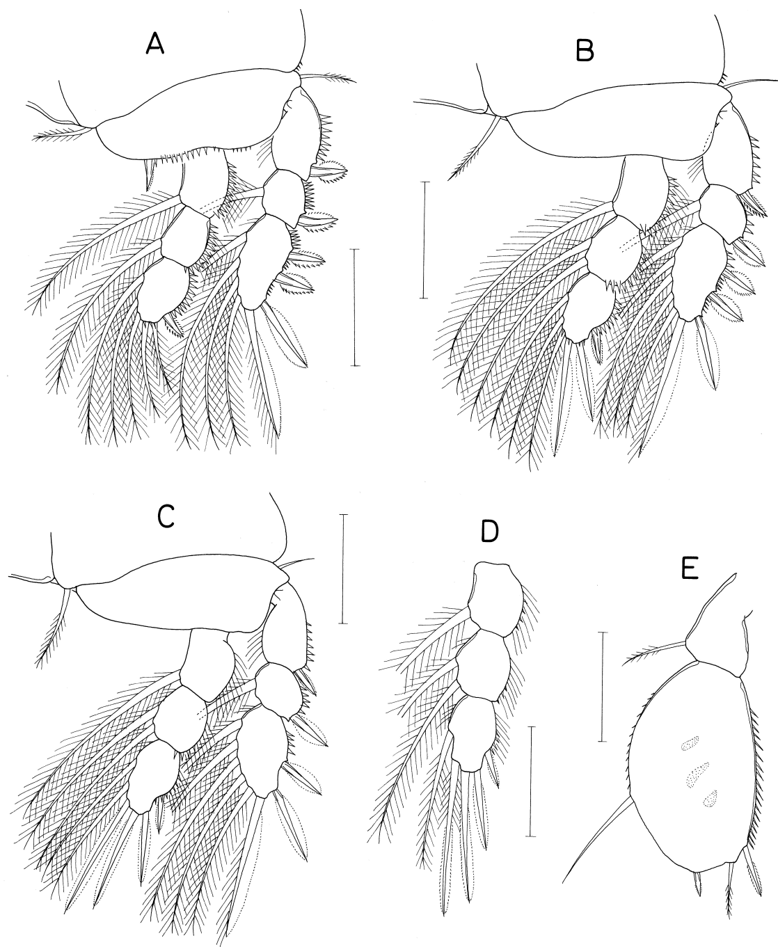
Fig. 65. Ostrincola binoviger n. sp., female. A, leg 1; B, leg 2; C, leg 3; D, endopod of leg 4; E, leg 5. Scales: 0.05 mm for all.
