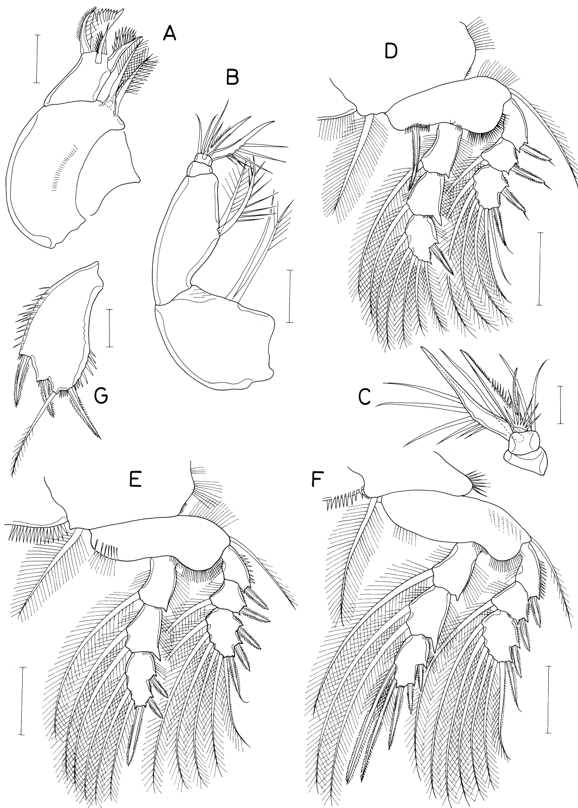
Fig. 15. Hemicyclops tripartitus n. sp., female. A, maxilla; B, maxilliped; C, distal part of maxilliped; D, leg 1; E, leg 2; F, leg 4; G, free segment of leg 5. Scales: A, B, G, 0.05 mm; C, 0.02 mm; D-F, 0.1 mm.
