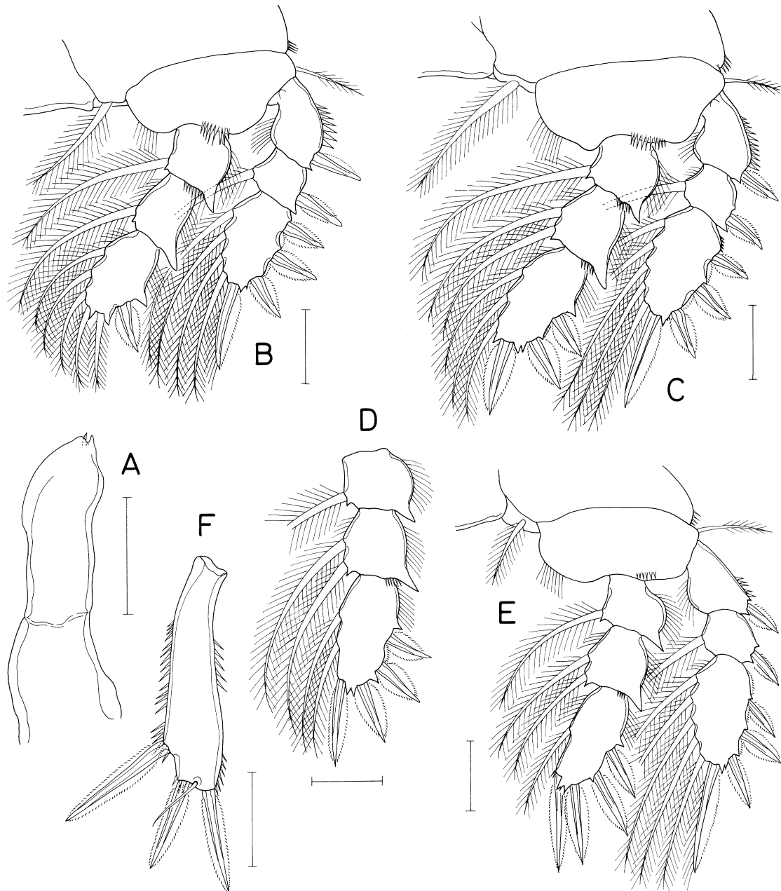
Fig. 2. Anthesius nosybensis n. sp., female. A, maxilliped; B, leg 1; C, leg 2; D, endopod of leg 3; E, leg 4; F, free segment of leg 5. Scales: 0.05 mm for all.
