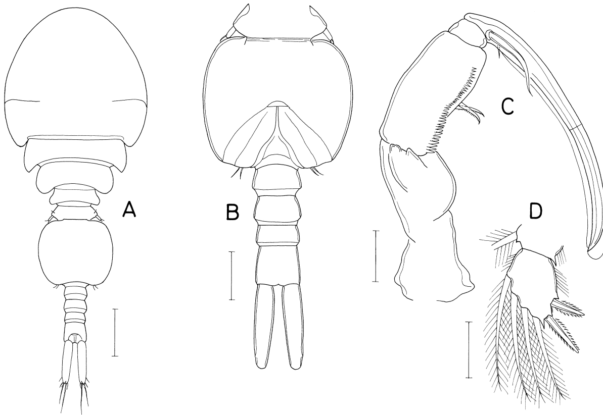
Fig. 31. Schedomolgus parvipediger n. sp., male. A, habitus, dorsal; B, urosome, ventral; C, maxilliped; D, third endopodal segment of leg 1. Scales: A, 0.2 mm; B, 0.1 mm; C, D, 0.05 mm.
