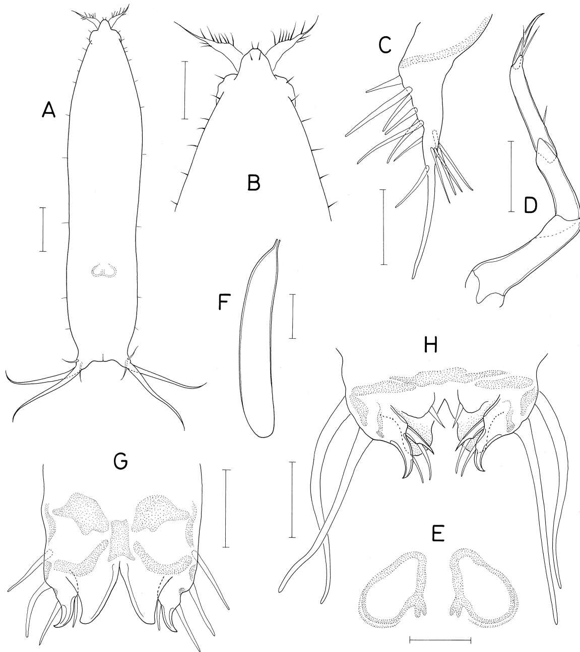
Fig. 61. Enalcyonium gradisetigerum n. sp. Female: A, habitus, dorsal; B, cephalic area, dorsal; C, antennule; D, antenna; E, genital areas; G, leg 1; H, leg 2. Male: F, spermatophore. Scales: A, 0.1 mm; B, F, 0.05 mm; C-E, G, H, 0.02 mm.
