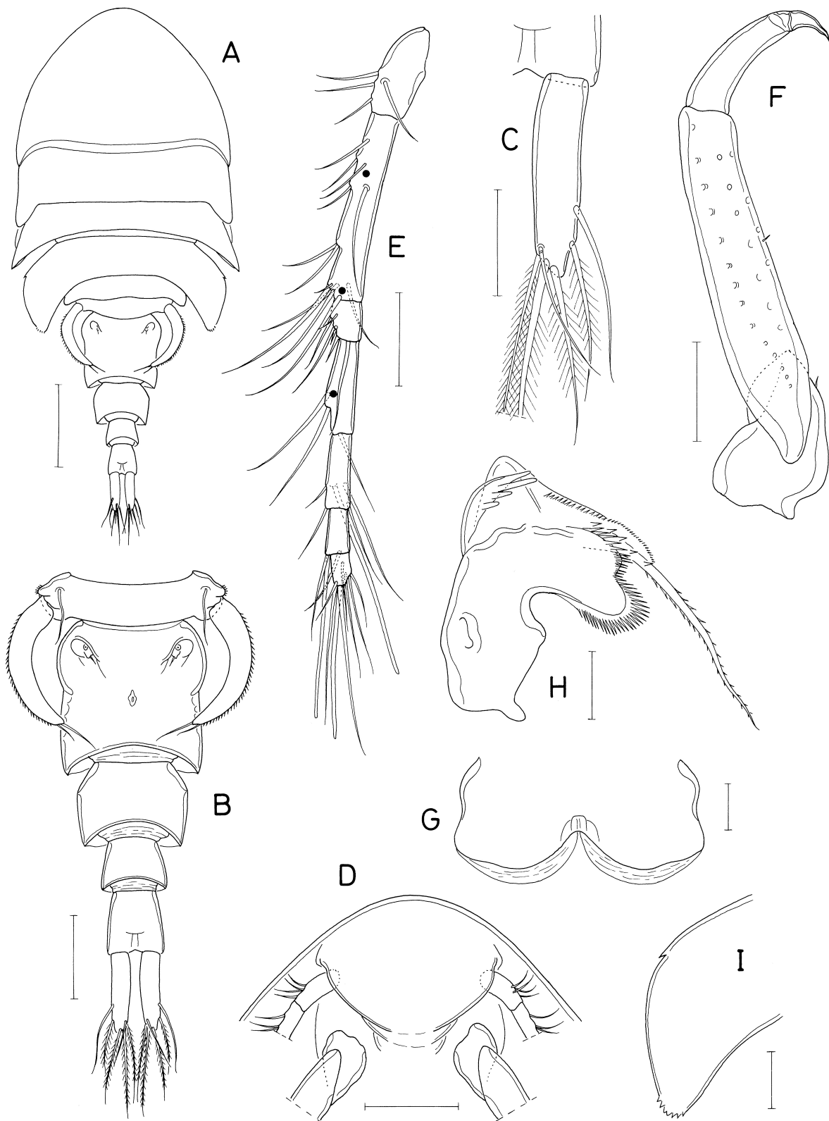
Fig. 26. Schedomolgus crenulatus n. sp., female. A, habitus, dorsal; B, urosome, dorsal; C, caudal ramus, dorsal; D, rostral area, ventral; E, antennule (dots indicating places of additional aesthetascs in male); F, antenna; G, labrum; H, mandible; I, epimera of third pedigerous somite. Scales: A, 0.2 mm; B, D, 0.1 mm; C, E, F, I, 0.05 mm; G, H, 0.02 mm.
