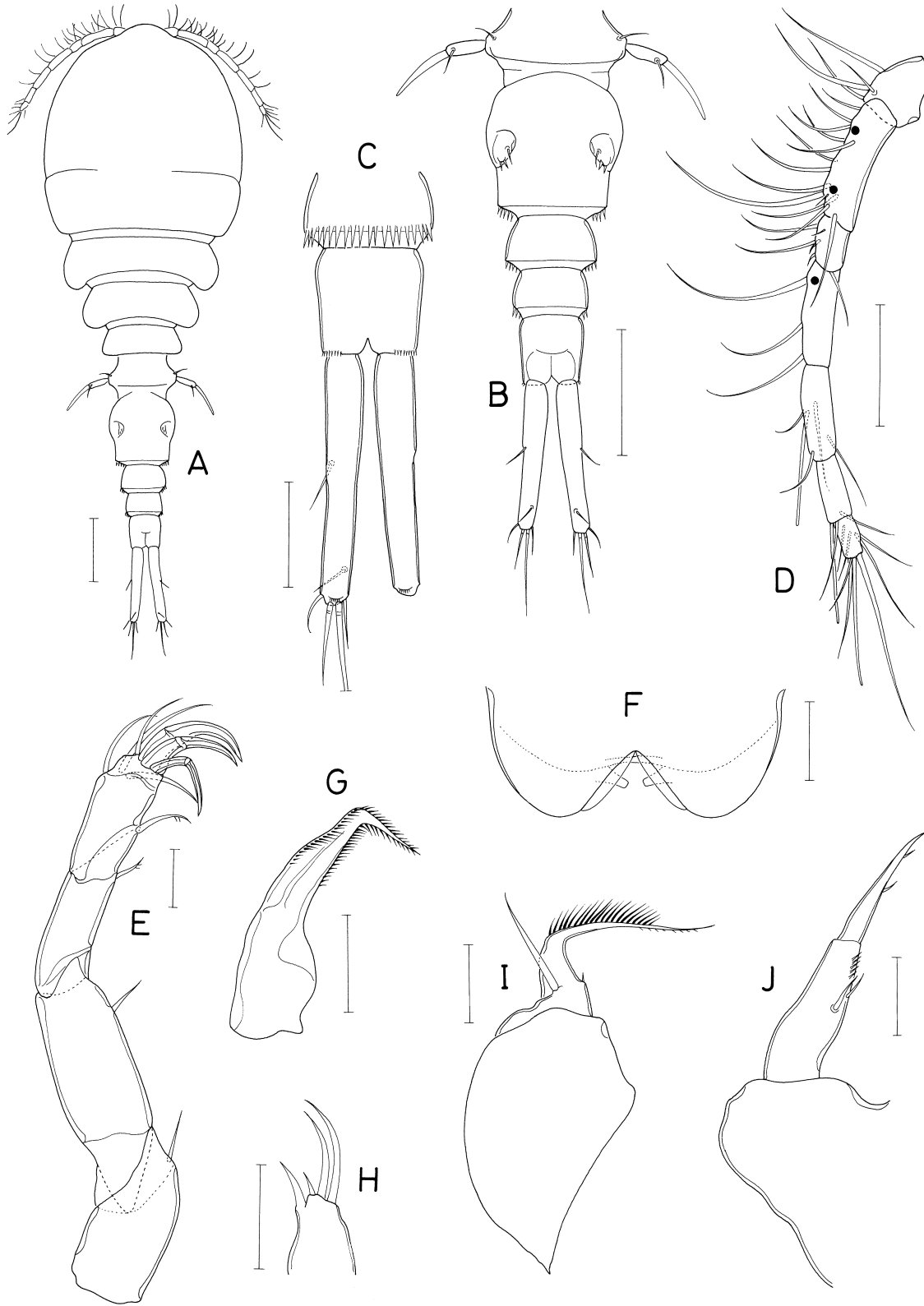
Fig. 41. Modiolicola trabalis Humes, female. A, habitus, dorsal; B, urosome, dorsal; C, distal part of abdomen, ventral; D, antennule (dots indicating places of additional aesthetascs in male); E, antenna; F, labrum; G, mandible; H, maxillule; I, maxilla; J, maxilliped. Scales: A, B, 0.1 mm; C, D, 0.05 mm; E-J, 0.02 mm.
