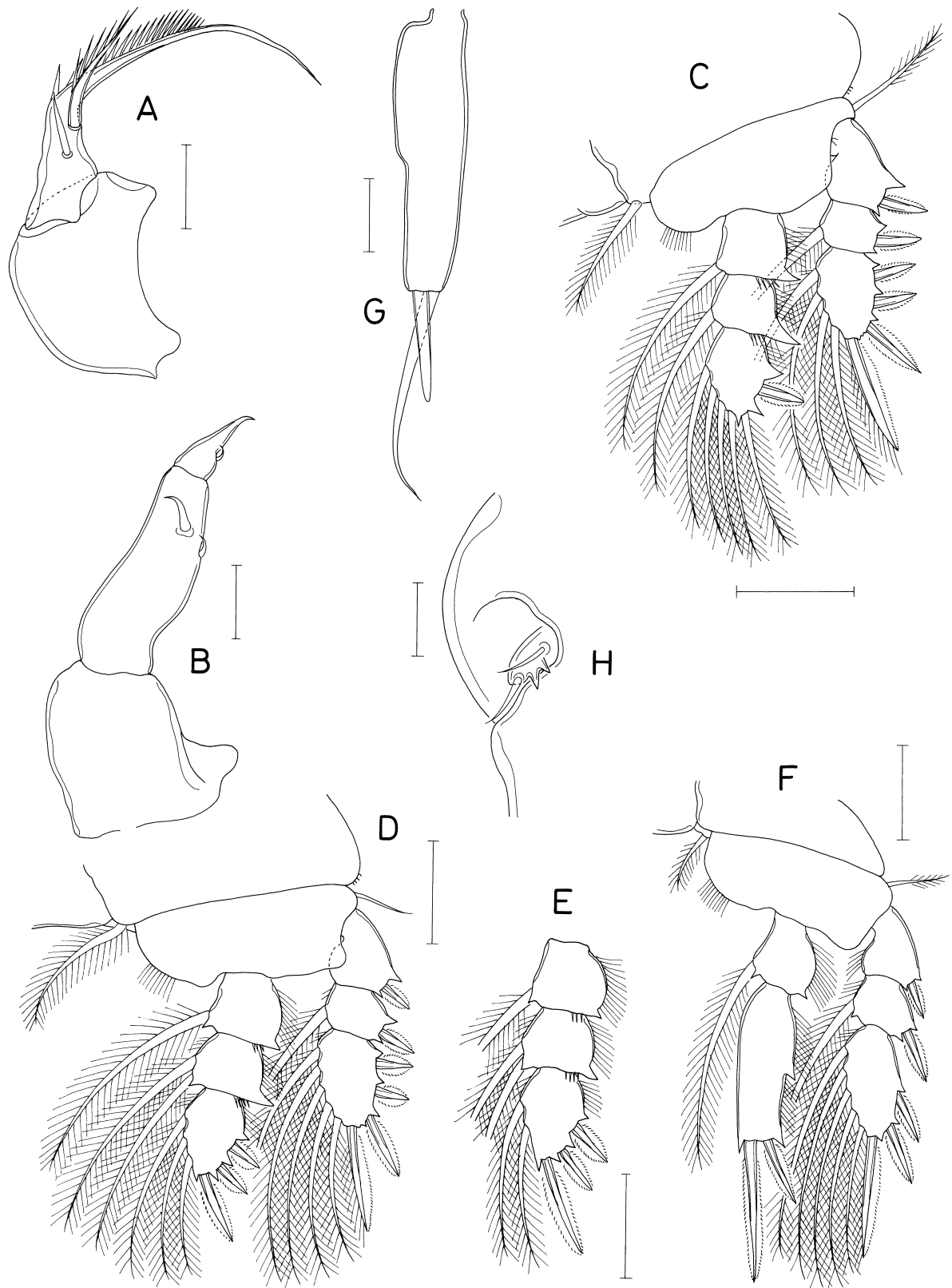
Fig. 36. Lichomolgus angustus n. sp., female. A, maxilla; B, maxillipe; C, leg 1; D, leg 2; E, endopod of leg 3; F, leg 4; G, free segment of leg 5; H, left genital area. Scales: A, B, G, H, 0.02 mm; C-F, 0.05 mm.
