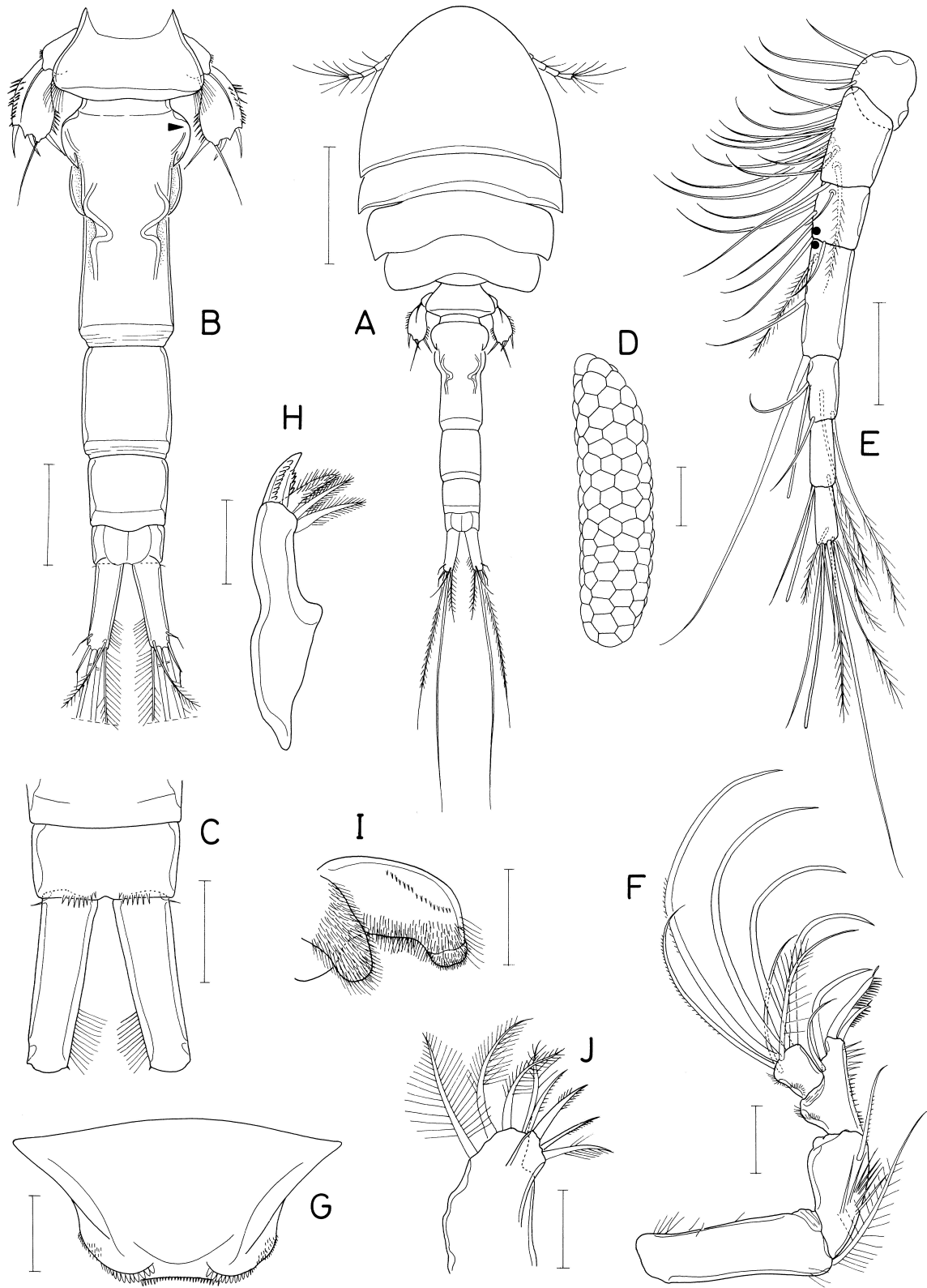
Fig. 14. Hemicyclops tripartitus n. sp., female. A, habitus, dorsal; B, urosome, dorsal; C, anal somite and caudal rami, ventral; D, egg sac; E, antennule; F, antenna; G, labrum, dorsal; H, mandible; I, paragnath; J, maxillule. Scales: A, 0.5 mm; B, D, 0.2 mm; C, E, 0.1 mm; F-J, 0.05 mm.
