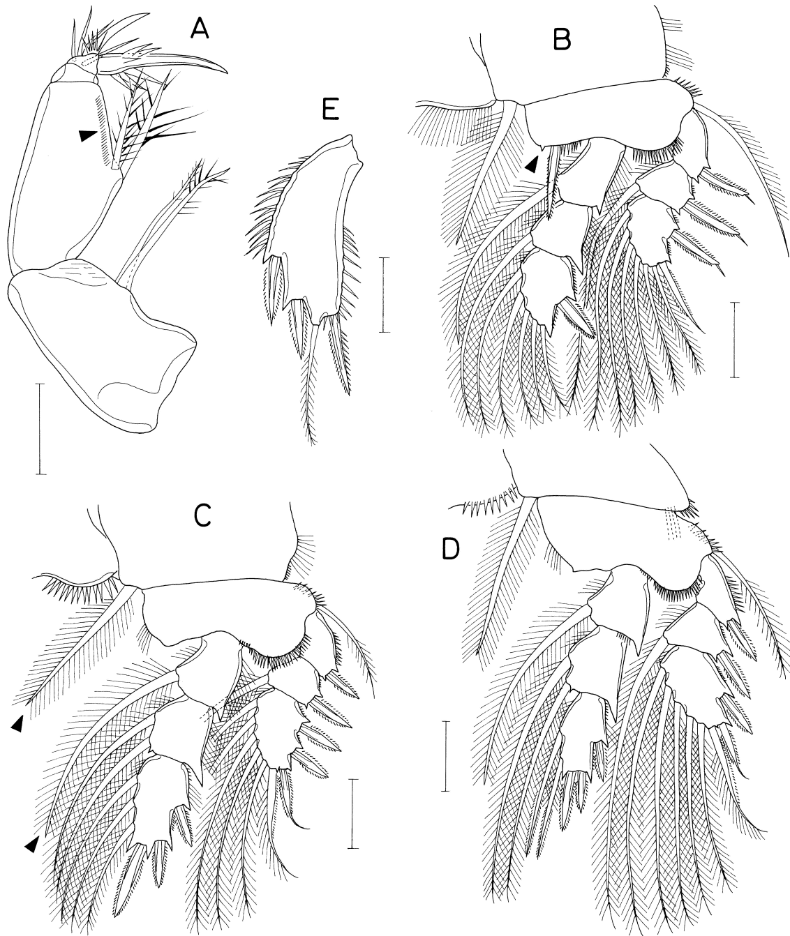
Fig. 11. Hemicyclops columnaris Humes, female. A, maxilliped; B, leg 1; C, leg 2; D, leg 4; E, free segment of leg 5. Scales: 0.05 mm for all.
