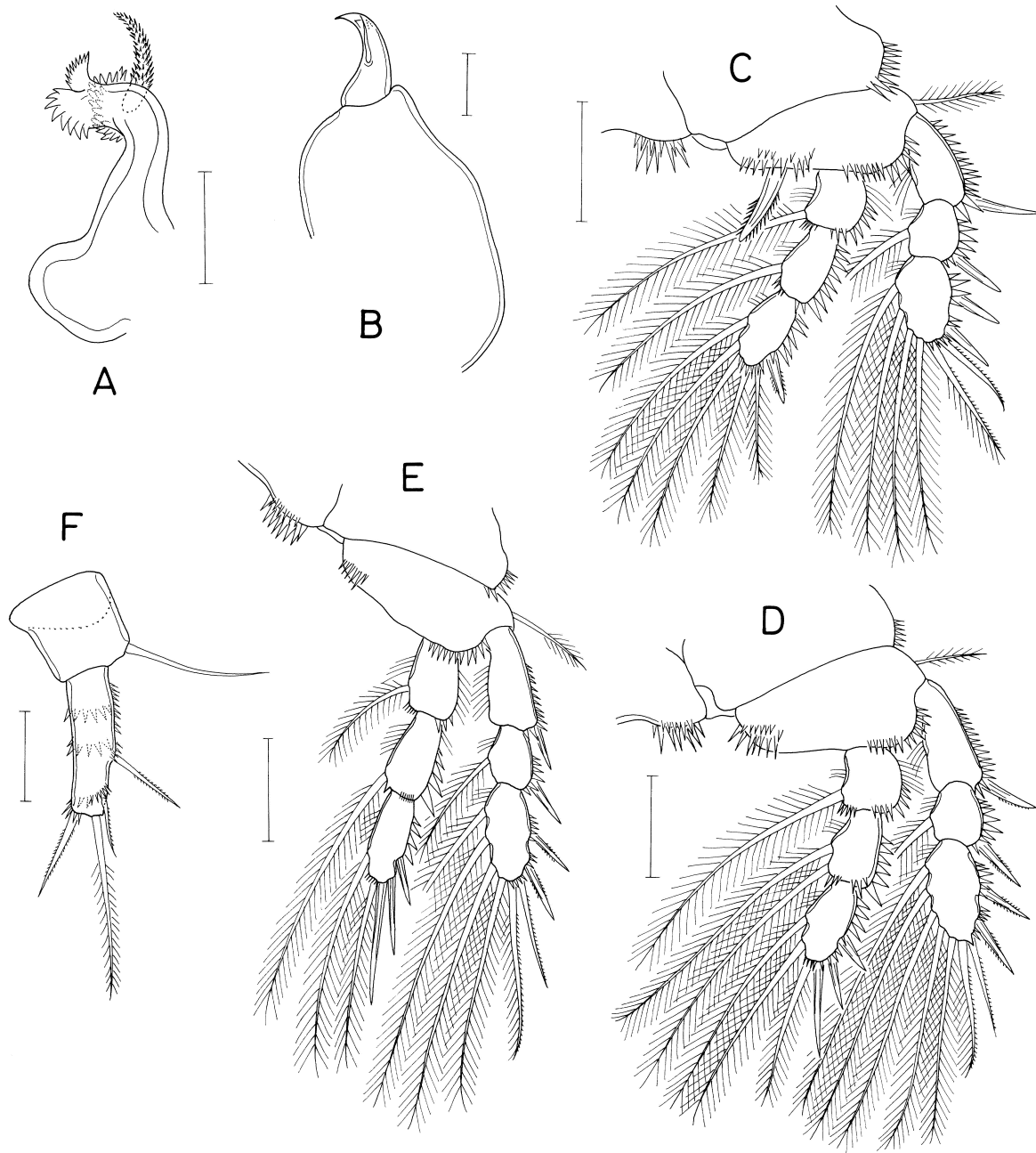
Fig. 24. Leptinogaster minuta n. sp., female. A, mandible; B, maxilla; C, leg 1; D, leg 2; E, leg 4; F, leg 5. Scales: A, B, 0.02 mm; C-G, 0.05 mm.
