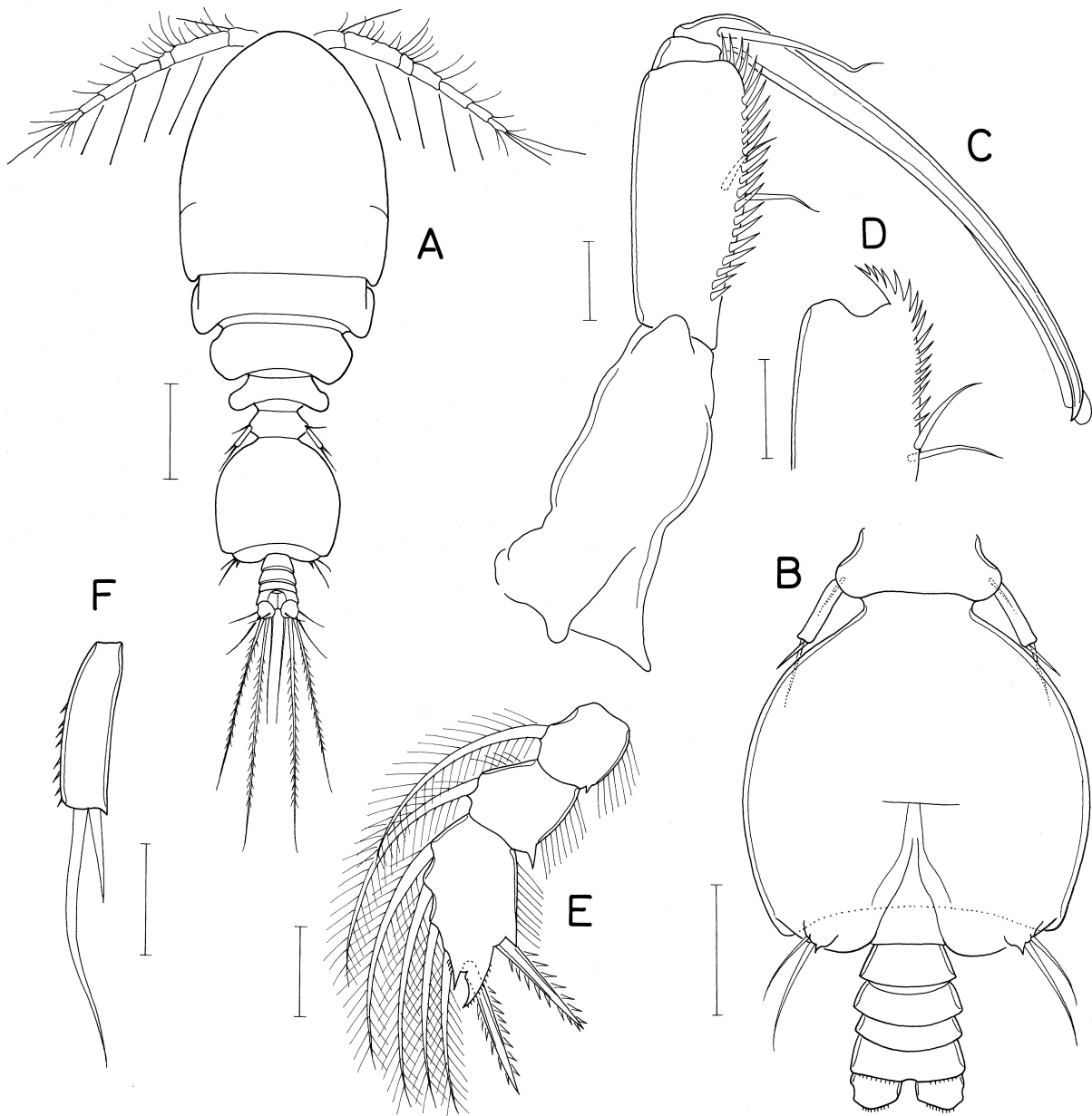
Fig. 52. Acanthomolgus tenuispinatus n. sp., male. A, habitus, dorsal; B, urosome, ventral; C, maxilliped; D, distal part of second segment of maxilliped; E, endopod of leg 1; F, free segment of leg 5. Scales: A, 0.1 mm; B, 0.05 mm; C-F, 0.02 mm.
