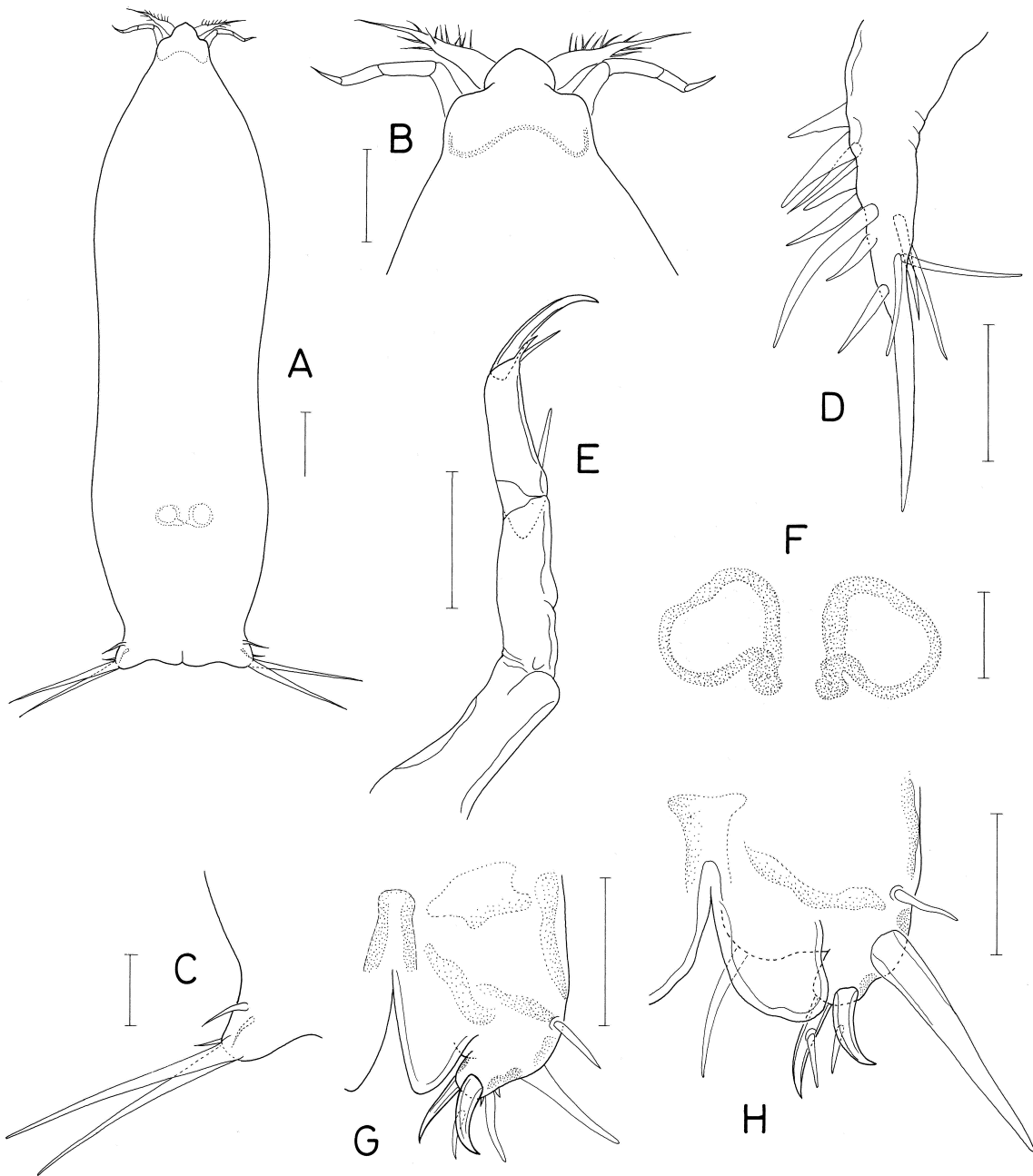
Fig. 60. Enalcyonium robustum n. sp., female. A, habitus, dorsal; B, cephalic area, dorsal; C, caudal ramus, dorsal; D, antennule; E, antenna; F, genital areas; G, leg 1; H, leg 2. Scales: A, 0.1 mm; B, C, 0.05 mm; D-H, 0.02 mm.
