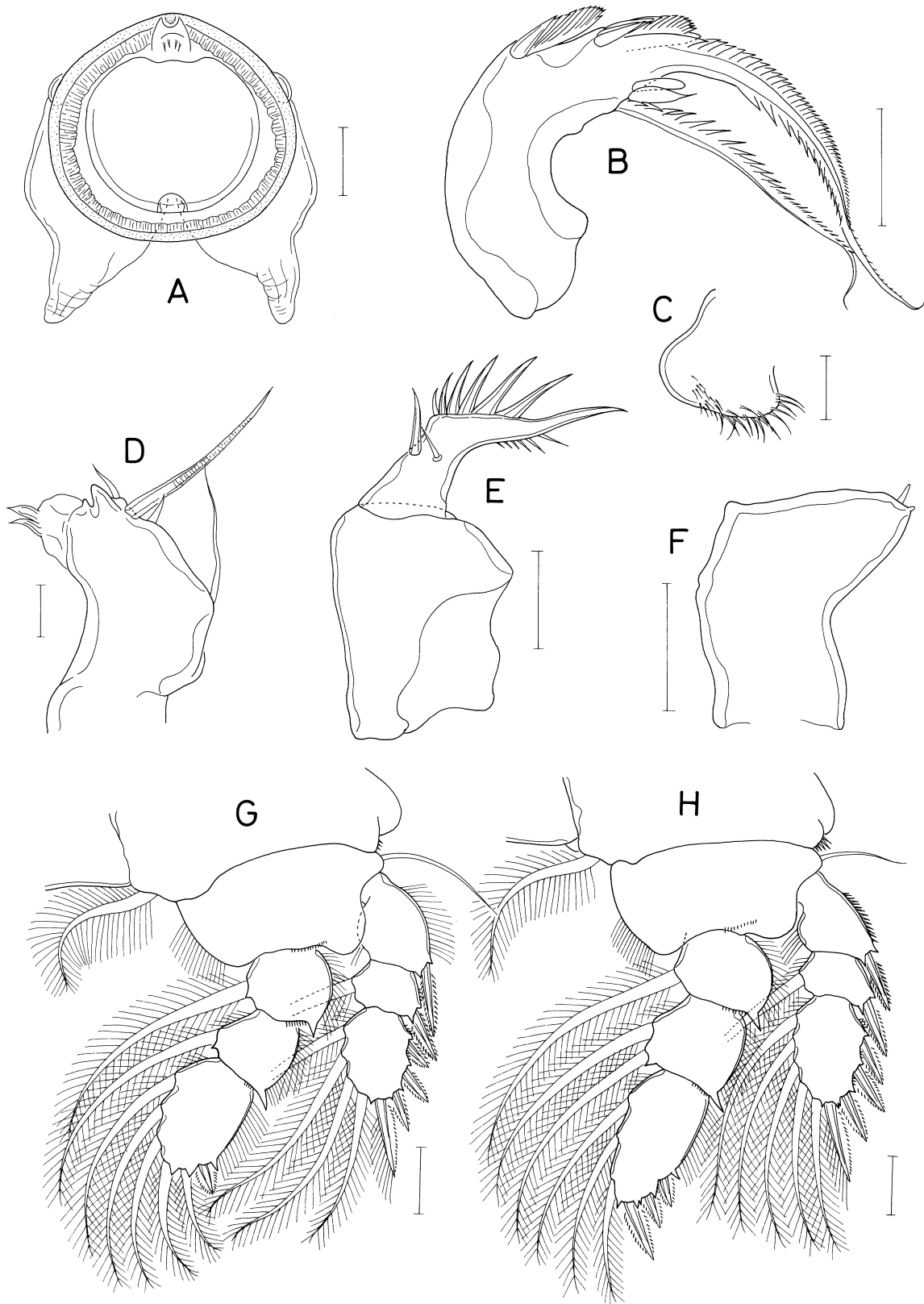
Fig. 5. Discantheissius solitarius n. gen. n. sp., female. A, labrum, ventral; B, mandible; C, paragnath; D, maxillule; E, maxilla; F, maxilliped; G, leg 1; H, leg 2. Scales: A, B, E-H, 0.05 mm; C, D, 0.02 mm.
