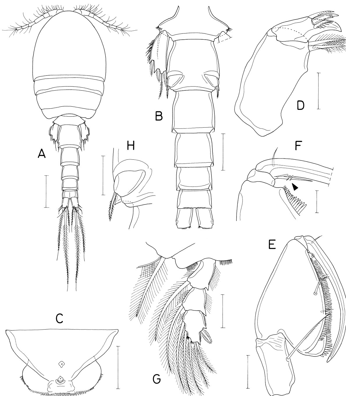
Fig. 12. Hemicyclops columnaris Humes, male. A, habitus, dorsal; B, urosome, ventral; C, labrum; D, maxilla; E, maxilliped; F, area of third segment of maxilliped; G, endopod of leg 1; H, genital area, ventral. Scales: A, 0.2 mm; B, 0.1 mm; C-E, G, H, 0.05 mm; F, 0.02 mm.
