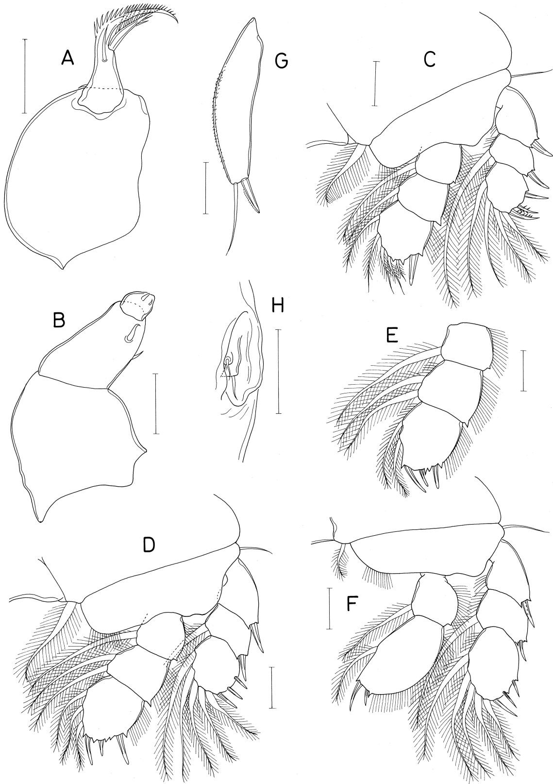
Fig. 54. Notoxynus lokobensis n. sp., female. A, maxilla; B, maxilliped; C, leg 1; D, leg 2; E, endopod of leg 3; F, leg 4; G, free segment of leg 5; H, right genital area. Scales: 0.05 mm for all.
