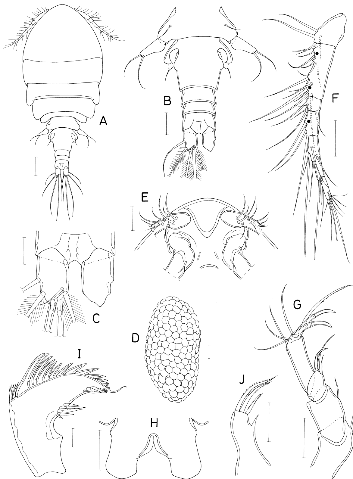
Fig. 32. Kellera multiovigera n. sp., female. A, habitus, dorsal; B, urosome, dorsal; C, caudal rami, dorsal; D, egg sac; E, rostral area, ventral; F, antennule (dots indicating places of additional aesthetascs in male); G, antenna; H, labrum; I, mandible; J, maxillule. Scales: A, 0.2 mm; B, D-H, 0.1 mm; C, J, 0.05 mm; I, 0.02 mm.
