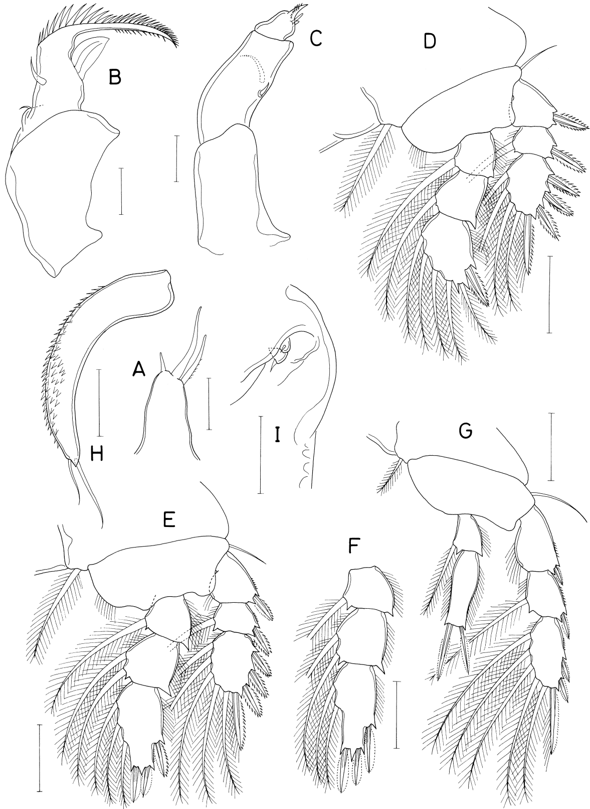
Fig. 27. Schedomolgus crenulatus n. sp., female. A, maxillule; B, maxilla; C, maxilliped; D, leg 1; E, leg 2; F, endopod of leg 3; G, leg 4; H, free segment of leg 5; I, right genital area, dorsal. Scales: A-C, 0.02 mm; D-I, 0.05 mm.
