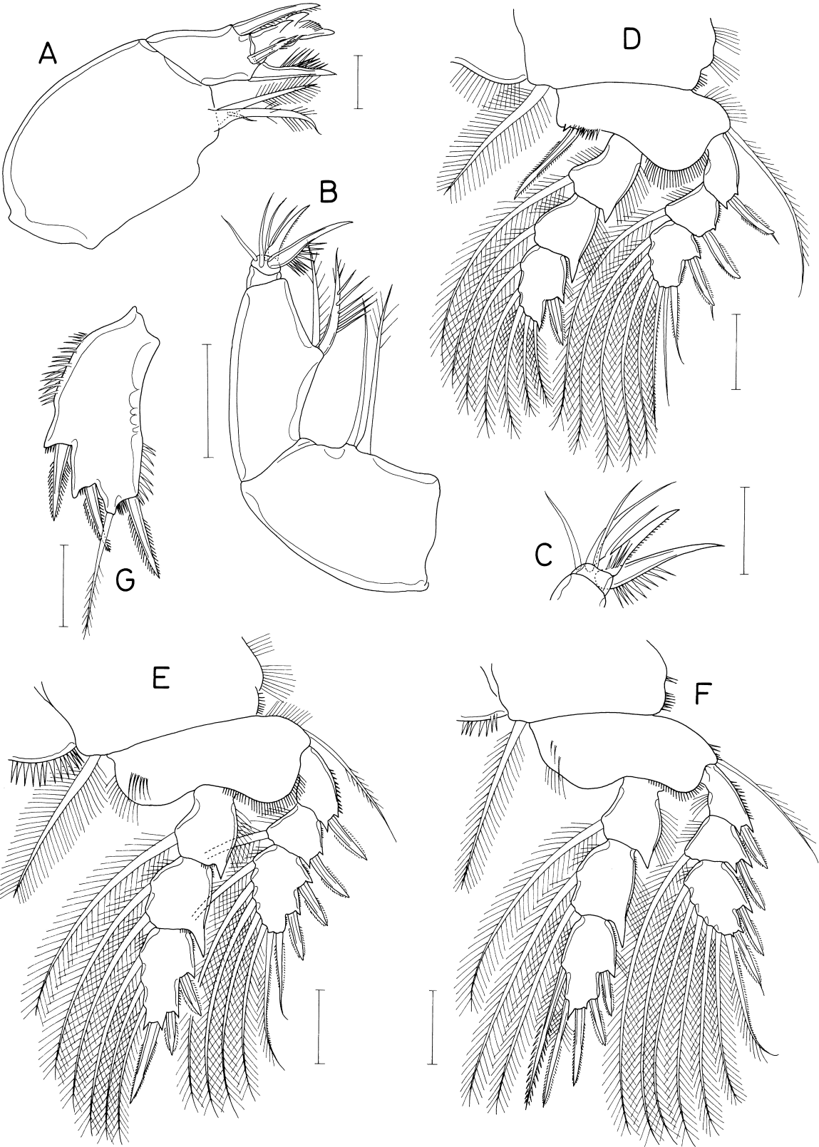
Fig. 21. Hemicyclops magnus n. sp., female. A, maxilla; B, maxilliped; C, distal part of maxilliped; D, leg 1; E, leg 2; F, leg 4; G, free segment of leg 5. Scales: A, 0.05 mm; B-G, 0.1 mm.
