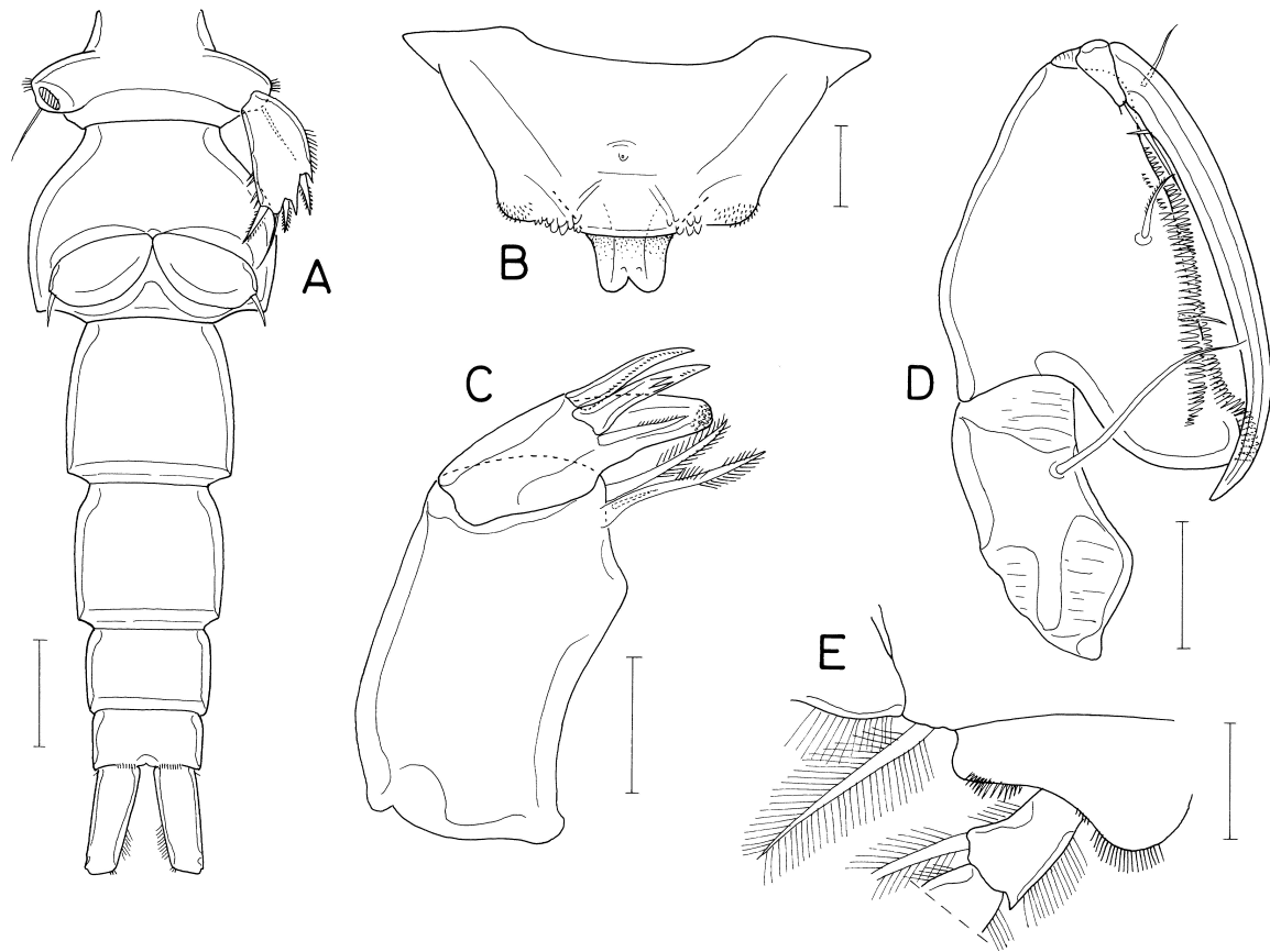
Fig. 22. Hemicyclops magnus n. sp., male. A, urosome, ventral; B, labrum, dorsal; C, maxilla; D, maxilliped; E, area near first endopodal segment of leg 1. Scales: A, 0.2 mm; B, 0.05 mm; C-E, 0.1 mm.
