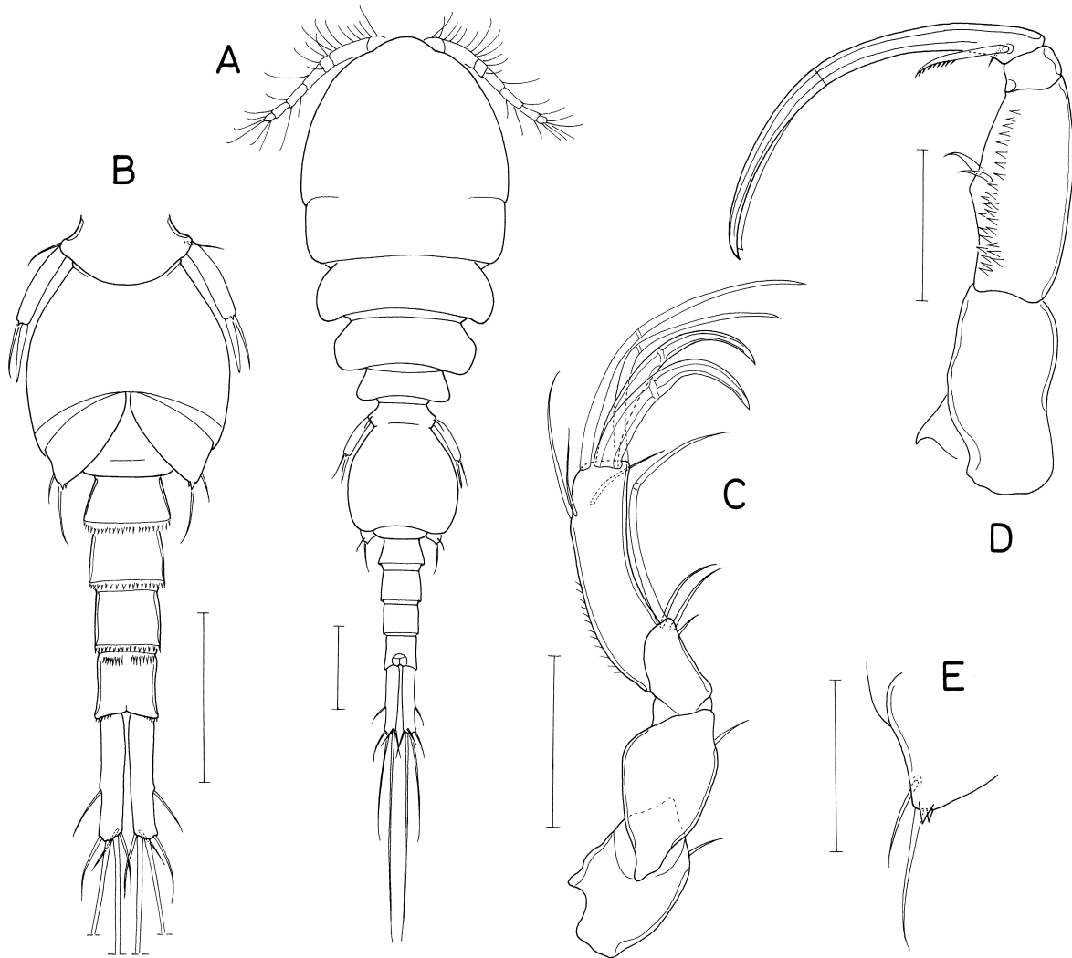
Fig. 37. Lichomolgus angustus n. sp., male. A, habitus, dorsal; B, urosome, ventral; C, antenna; D, maxilliped; E, posterodistal corner of genital somite, ventral. Scales: A, B, 0.1 mm; C-E, 0.05 mm.
