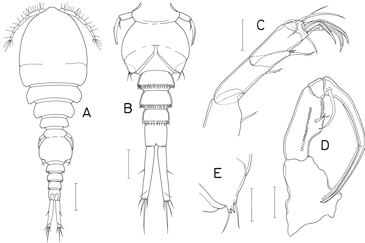
Fig. 43. Modiolicola trabalis Humes, male. A, habitus, dorsal; B, urosome, ventral; C, distal part of antenna; D, maxilliped; E, postero-distal part of genital somite, ventral. Scales: A, 0.1 mm; B, 0.05 mm; C-E, 0.02 mm.
