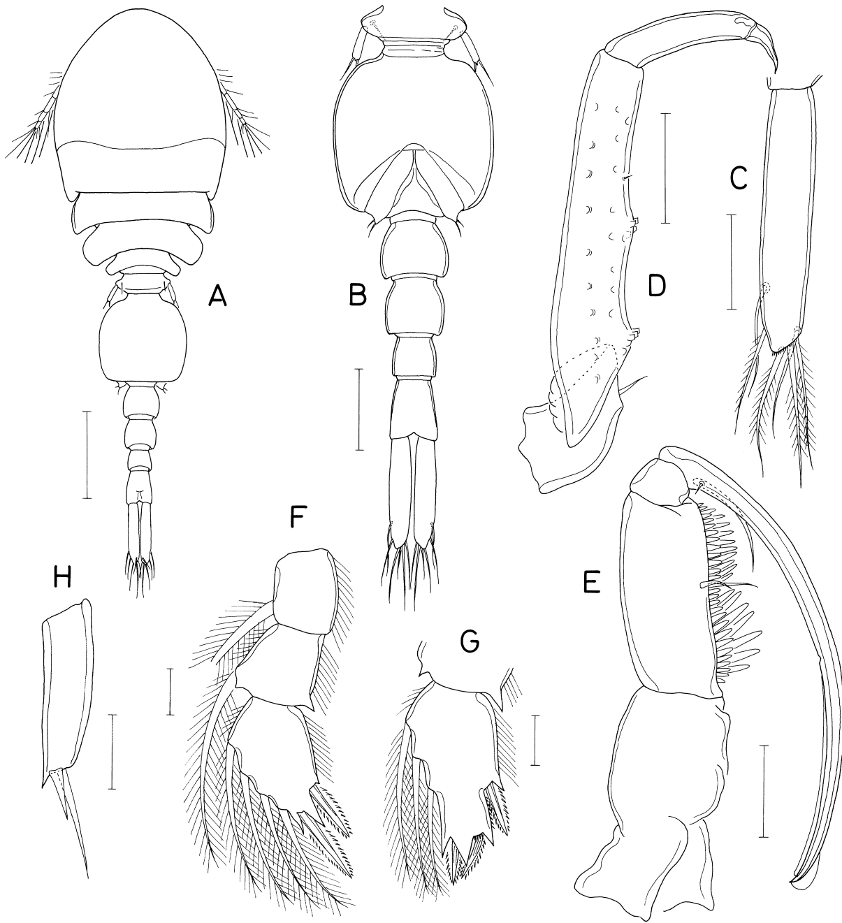
Fig. 28. Schedomolgus crenulatus n. sp., male. A, habitus, dorsal; B, urosome, ventral; C, right caudal ramus, ventral; D, antenna; E, maxilliped; F, endopod of leg 1; G, third endopodal segment of leg 2; H, free segment of leg 5. Scales: A, 0.2 mm; B, 0.1 mm; C-E, 0.05 mm; F-H, 0.02 mm.
