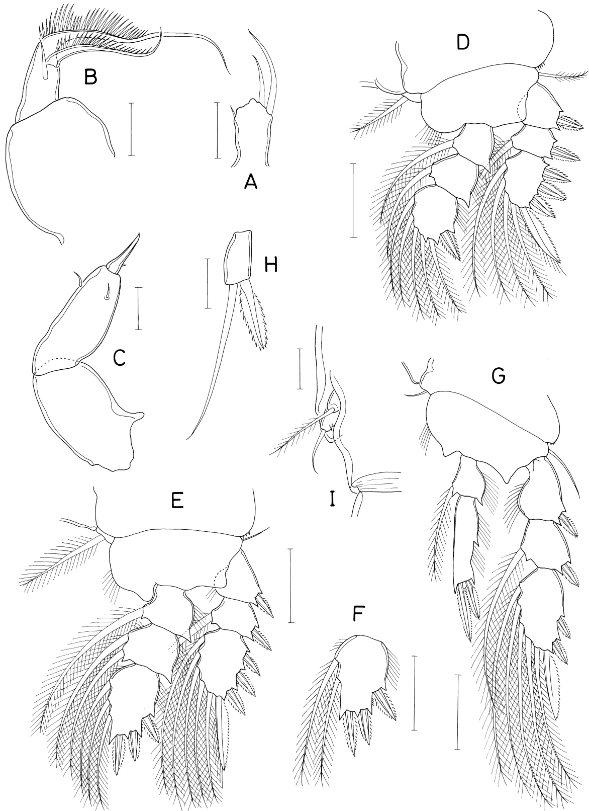
Fig. 39. Lichomolgus fusiformis n. sp., female. A, maxillule; B, maxilla; C, maxilliped; D, leg 1; E, leg 2; F, third endopodal segment of leg 3; G, leg 4; H, free segment of leg 5; I, left genital area, dorsal. Scales: A-C, H, I, 0.02 mm; D-G, 0.05 mm.
