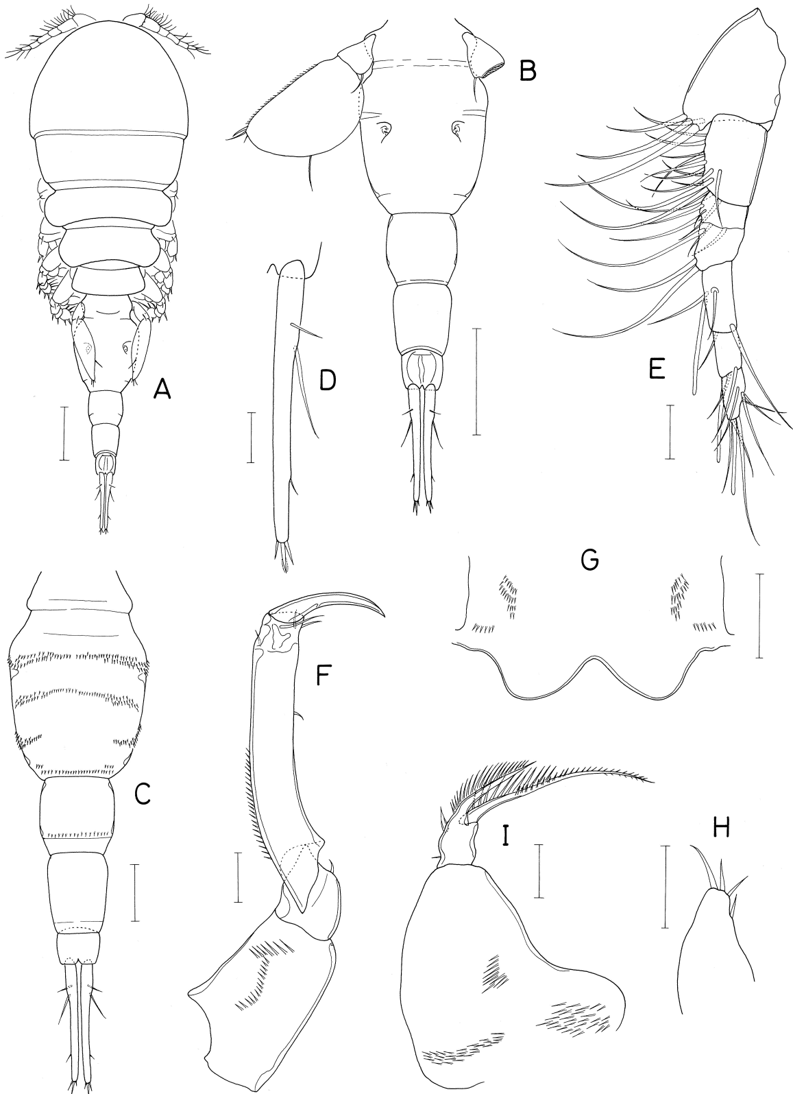
Fig. 62. Ostrincola breviseti Ho and Kim, female. A, habitus, dorsal; B, urosome, dorsal; C, urosome, ventral; D, right caudal ramus, dorsal; E, antennule; F, antenna; G, labrum; H, maxillule; I, maxilla. Scales: A, B, 0.1 mm; C, G, 0.05 mm; D-F, H, I, 0.02 mm.
