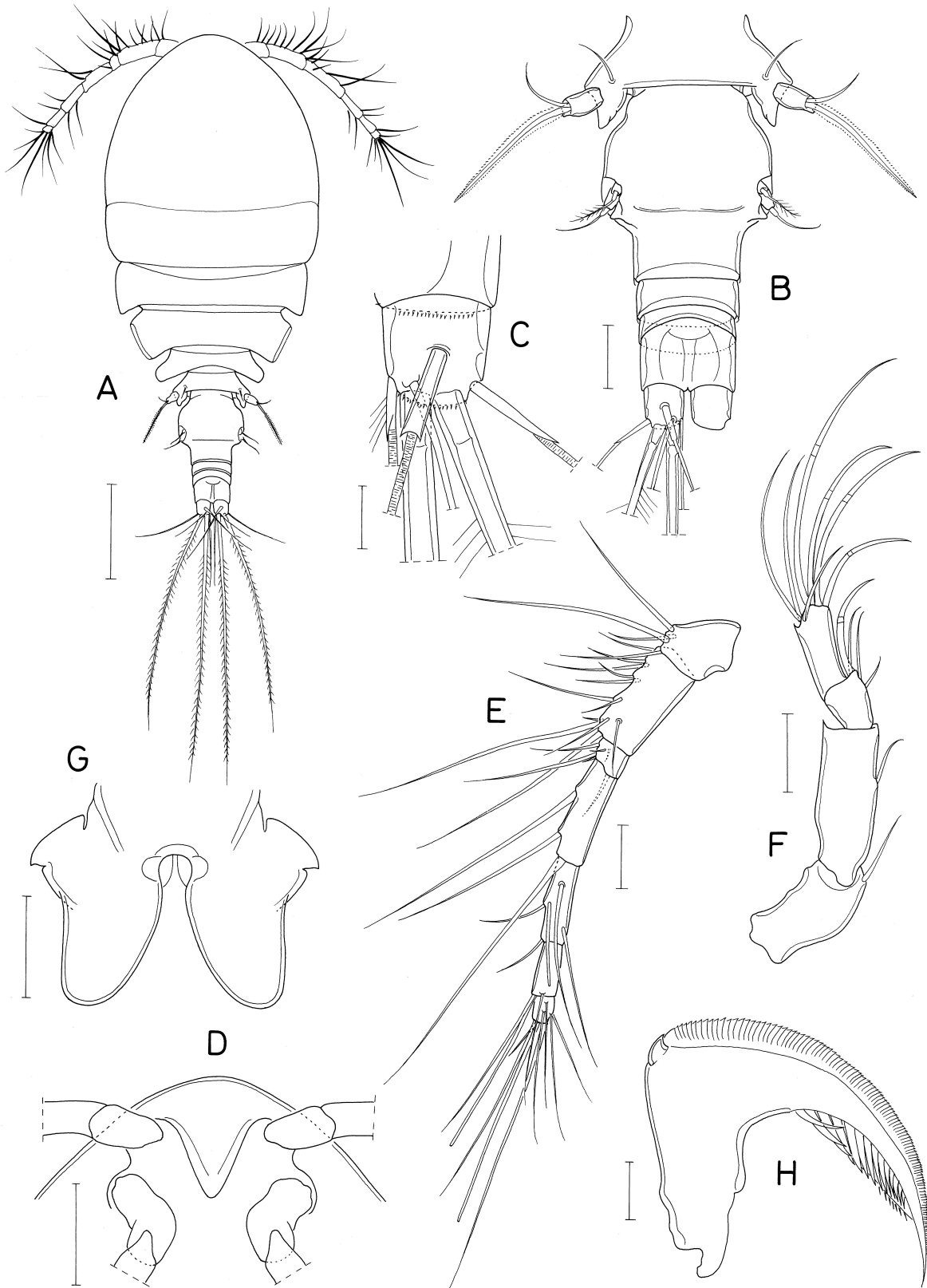
Fig. 58. Eupolymniphilus brevicaudatus n. sp., female. A, habitus, dorsal; B, urosome, dorsal; C, right caudal ramus, dorsal; D, rostral area, ventra; E, antennule; F, antenna; G, labrum; H, mandible. Scales: A, 0.2 mm; B, D-G, 0.05 mm; C, H, 0.02 mm.
