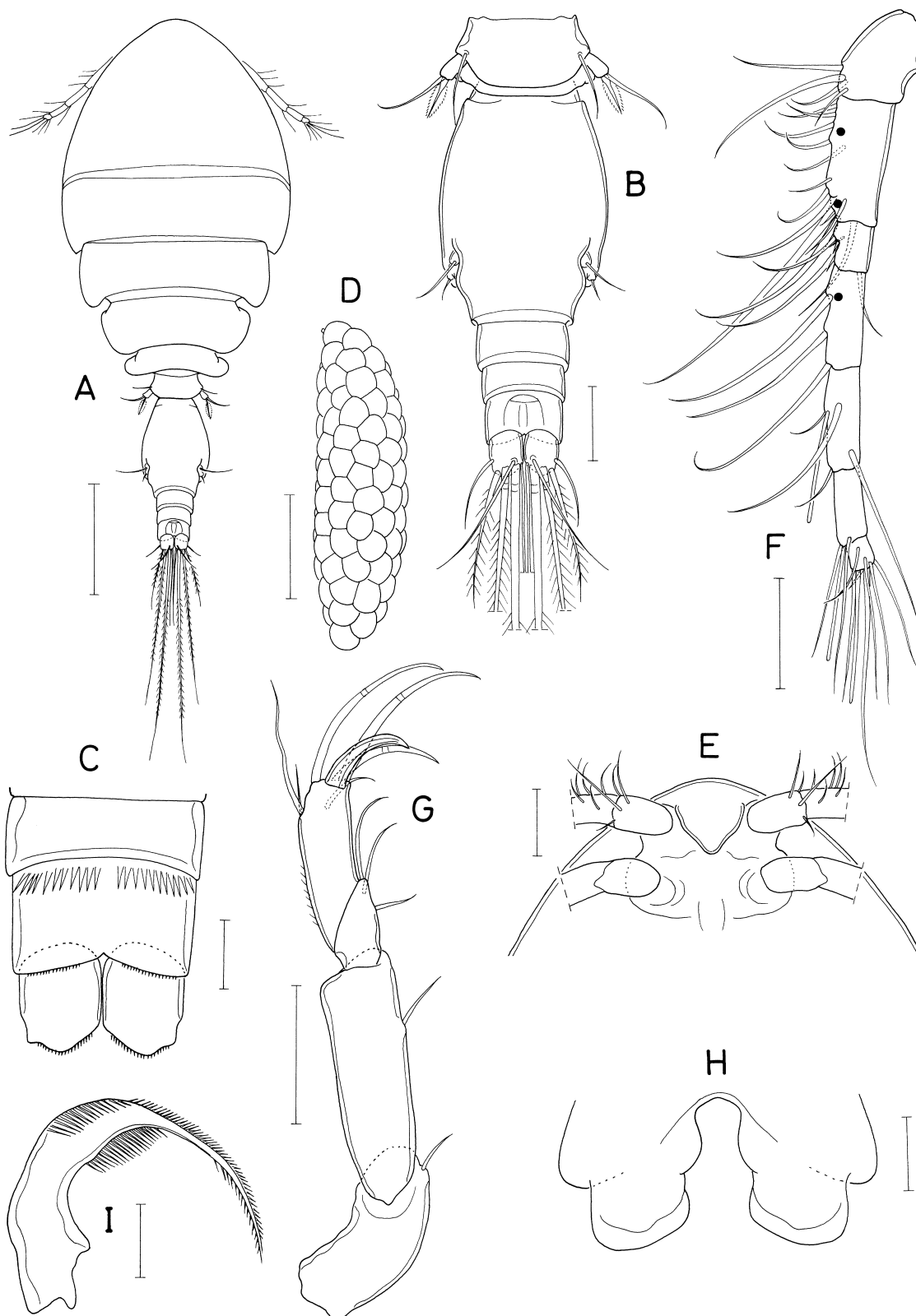
Fig. 38. Lichomolgus fusiformis n. sp., female. A, habitus, dorsal; B, urosome, dorsal; C, distal part of abdomen, ventral; D, egg sac; E, rostral area, ventral; F, antennule (dots indicating places of additional aesthetascs in male); G, antenna; H, labrum; I, mandible. Scales: A, D, 0.2 mm; B, E-G, 0.05 mm; C, H, I, 0.02 mm.
