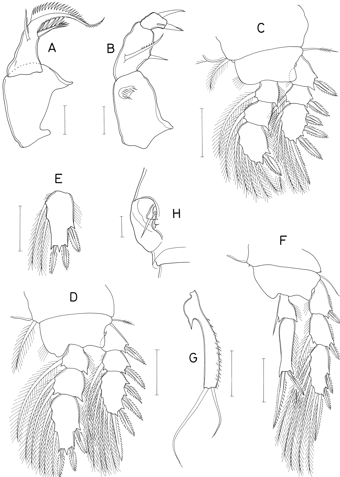
Fig. 51. Acanthomolgus tenuispinatus n. sp., female. A, maxilla; B, maxilliped; C, leg 1; D, leg 2; E, third endopodal segment of leg 3; F, leg 4; G, free segment of leg 5; H, left genital area, dorsal. Scales: A, B, H, 0.02 mm; C-G, 0.05 mm.
