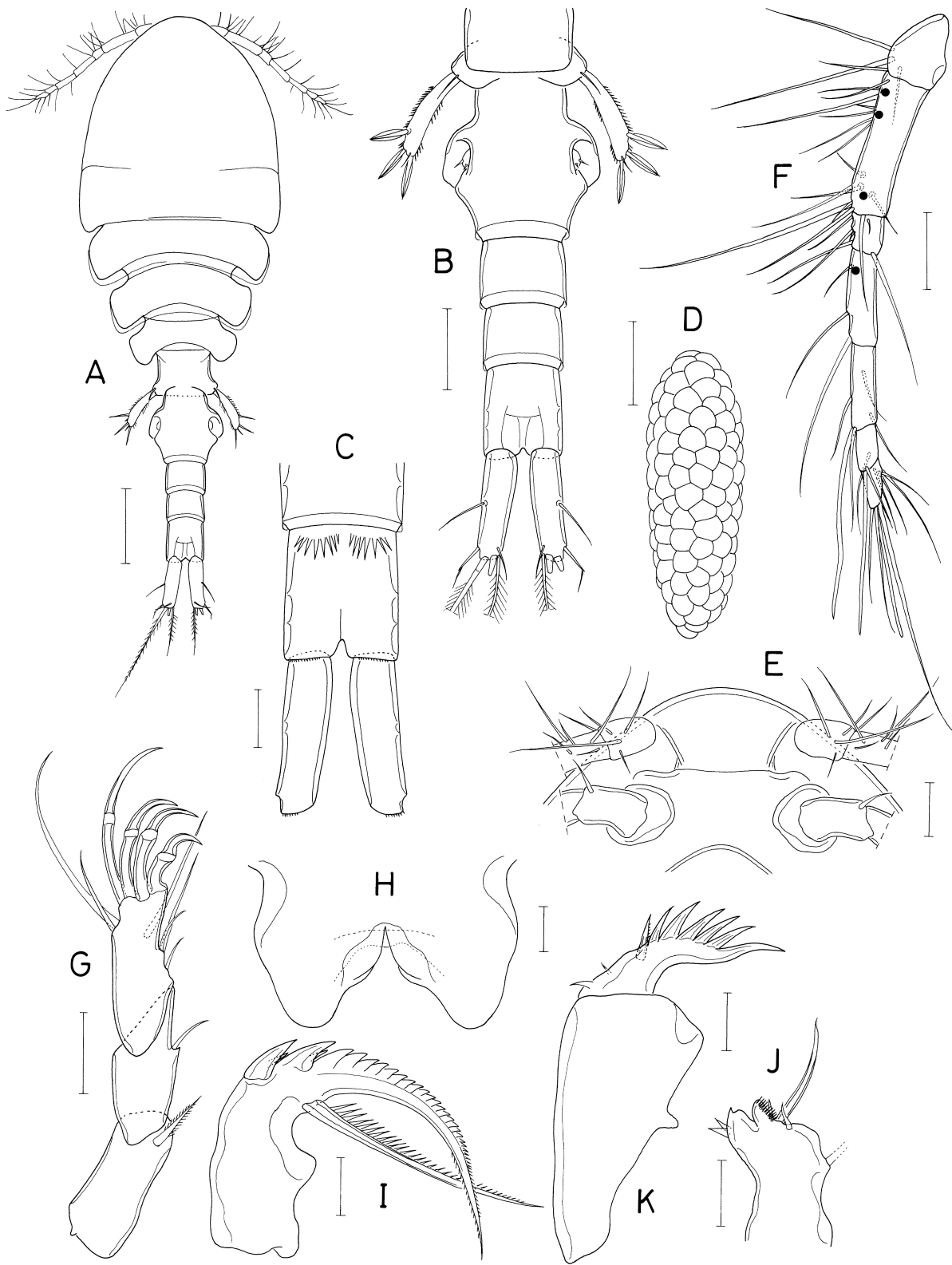
Fig. 1. Anthessius nosybensis n. sp., female. A, habitus, dorsal; B, urosome, dorsal; C, distal part of abdomen, ventral; D, egg sac; E, rostral area, ventral; F, antennule (dots indicating places of additional aesthetascs in male); G, antenna; H, labrum; I, mandible; J, maxillule; K, maxilla. Scales: A, D, 0.2 mm; B, 0.1 mm; C-G, 0.05 mm; H-K, 0.02 mm.
