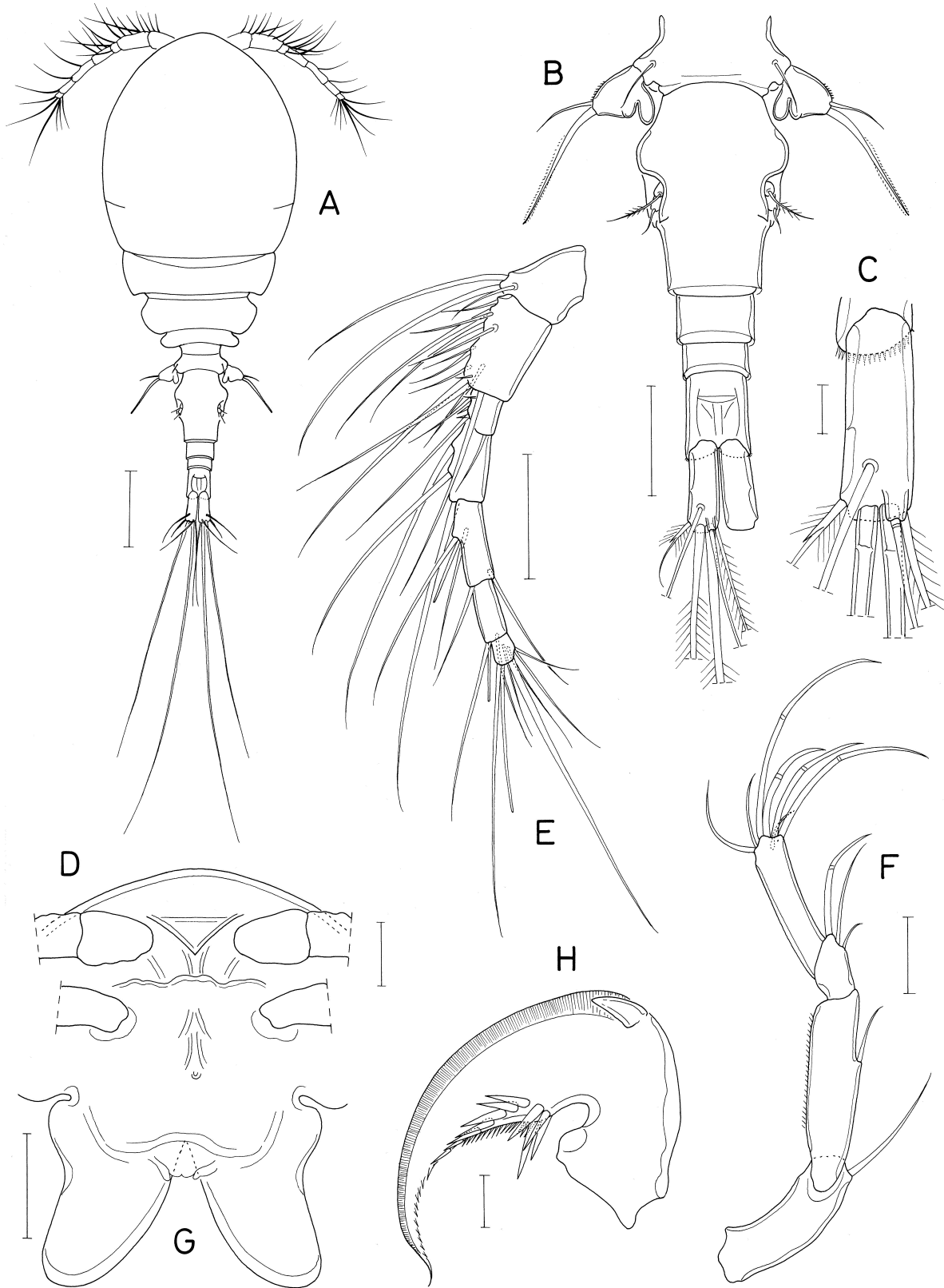
Fig. 48. Tubiporicola inflatus n. sp., female. A, habitus, dorsal; B, urosome, dorsal; C, left caudal ramus, dorsal; D, rostral area, ventral; E, antennule; F, antenna; G, labrum; H, mandible. Scales: A, 0.2 mm; B, E, 0.1 mm; C, H, 0.02 mm; D, F, G, 0.05 mm.
